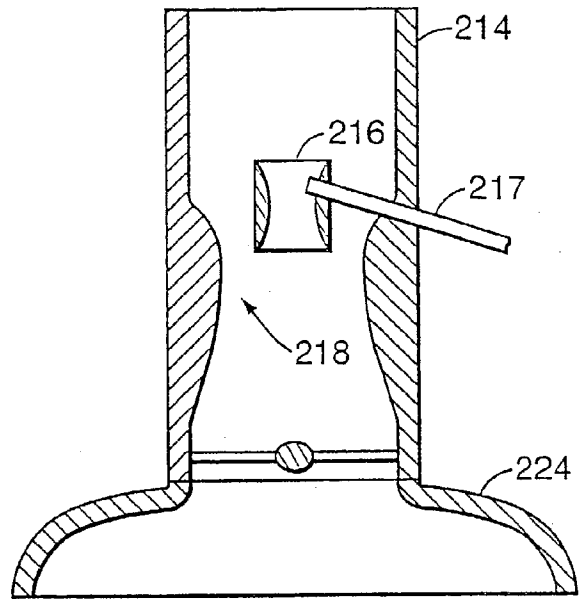
FIG. 15 PRIOR ART
