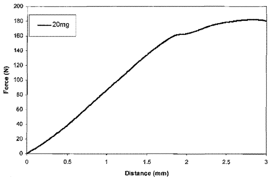
Example 20 Indentation Test of Example 14.3 tablet
