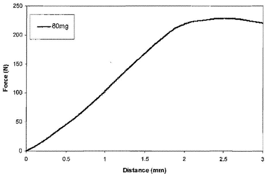
Example 20 Indentation Test of Example 16.2 tablet
