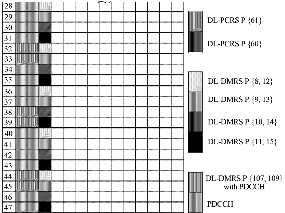
FIG. 2B-2 (PRIOR ART)
