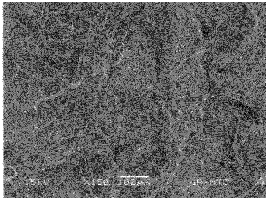
FIG. 4A 50% MICROFIBER, YANKEE SIDE
