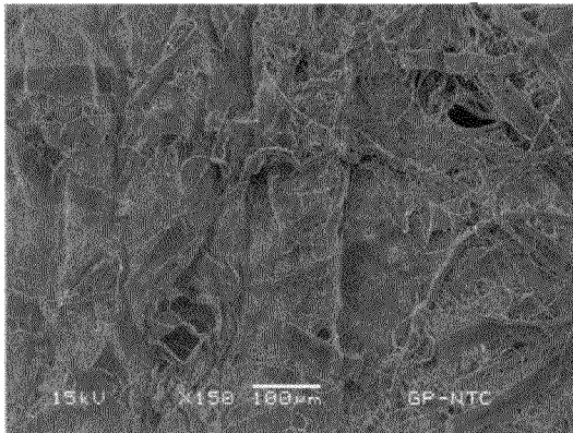
FIG. 3A 50% MICROFIBER, AIR SIDE
