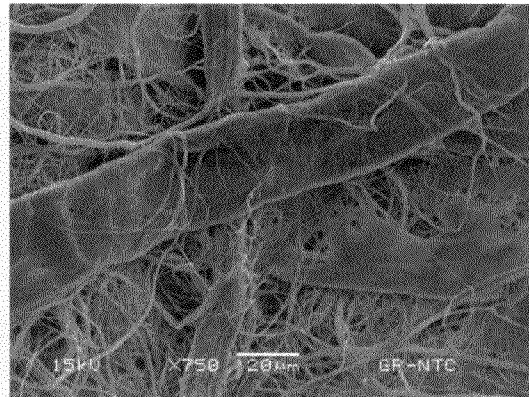
FIG. 3B 50% MICROFIBER, AIR SIDE
