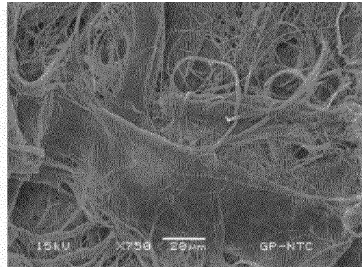
FIG. 4B 50% MICROFIBER, YANKEE SIDE
