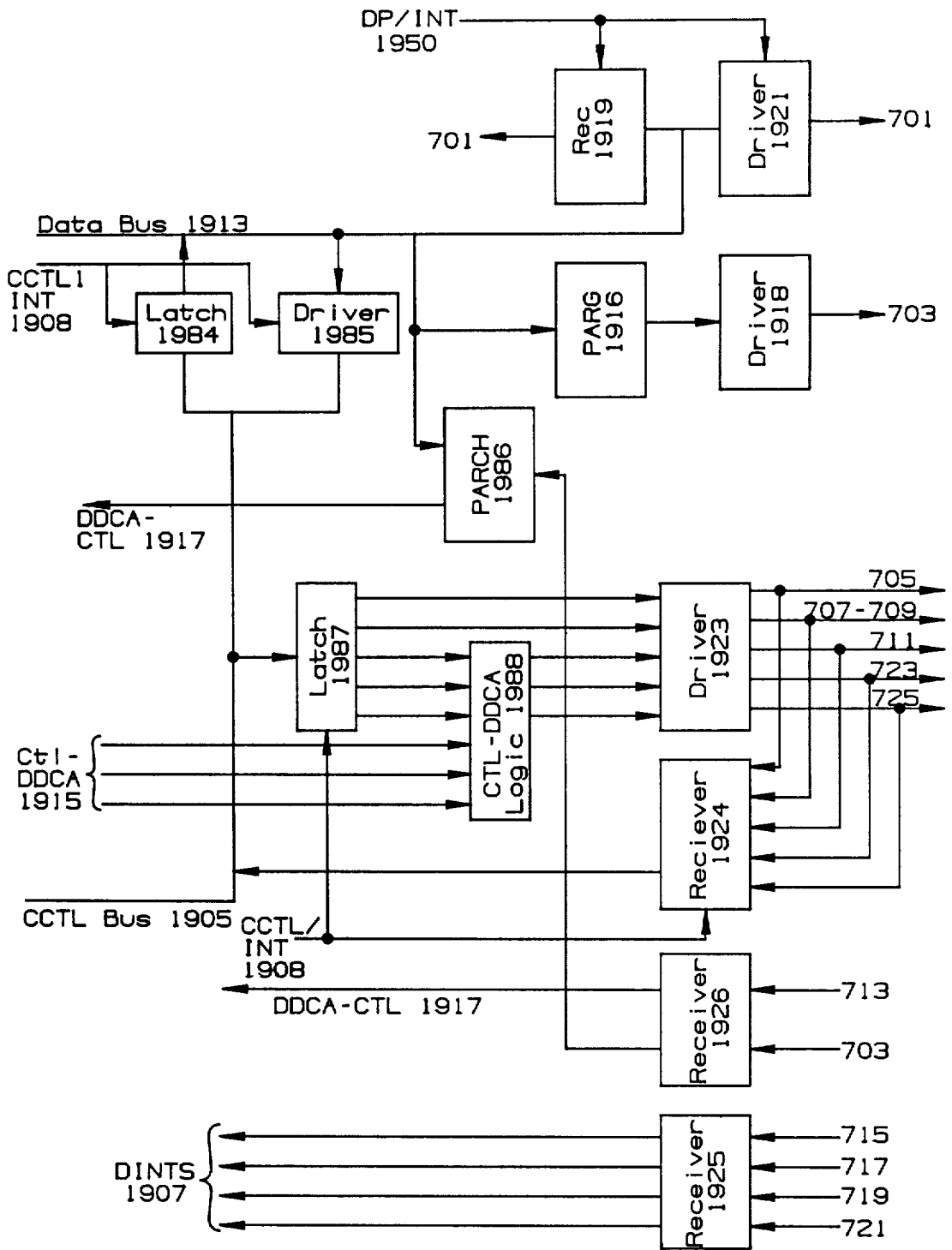
Disk Interface 1929 Detail
