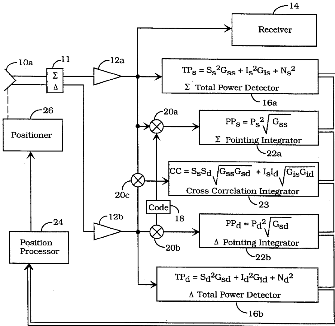
Closed Loop Receive Antenna
