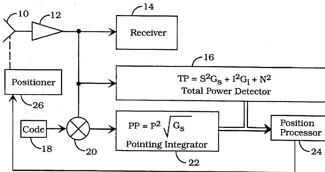
Open Loop Receive Antenna
