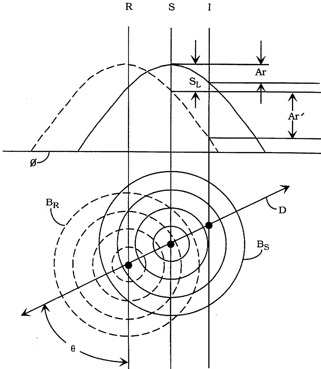
Beam Repositioning Technique
