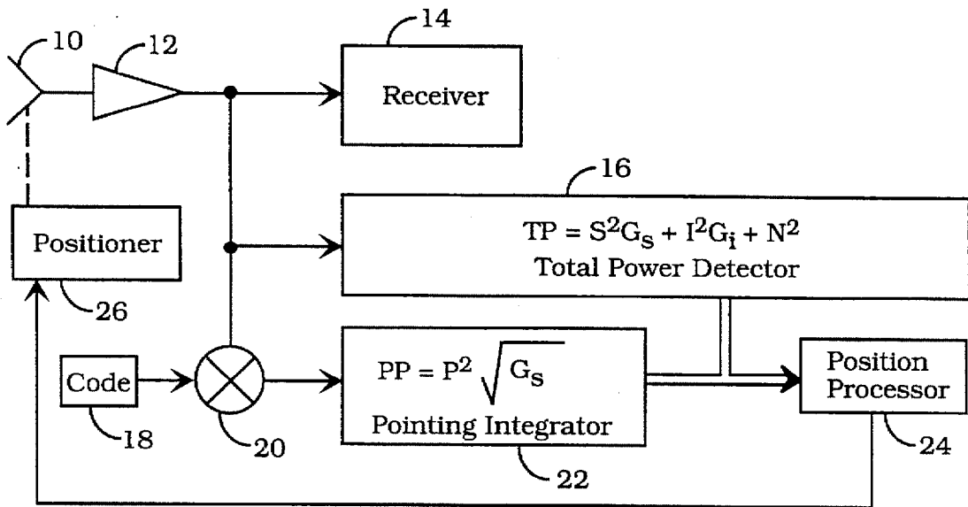
Open Loop Receive Antenna
