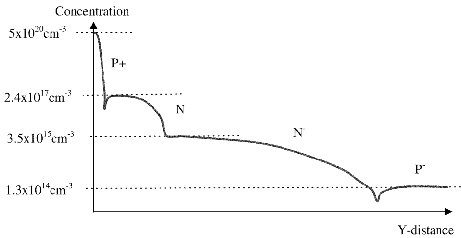
a) State of the art LIGBT
