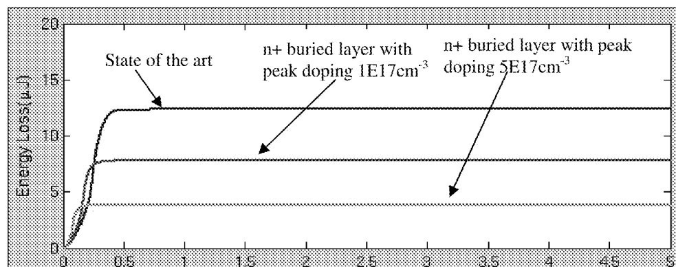
i) Energy loss
