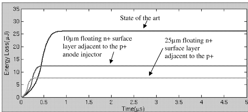
f) Energy loss
