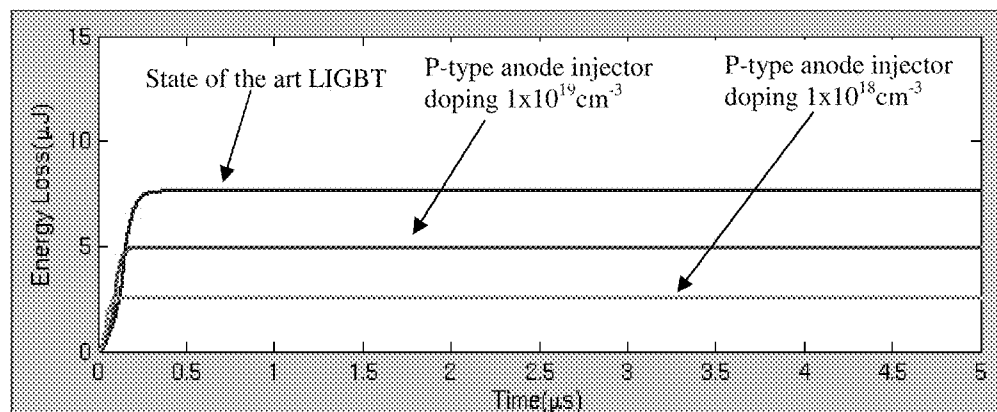
c) Energy loss FIG. 8
