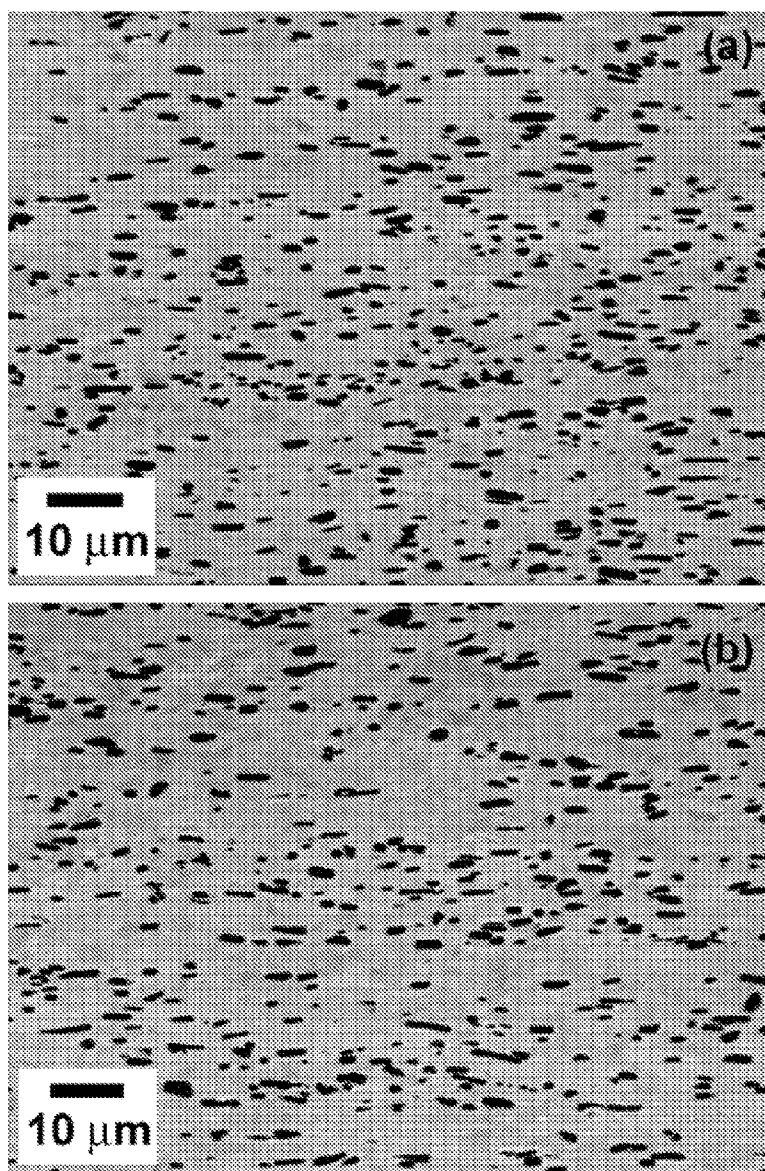
FIG. 23 Backscattered SEM images of microstructure in Alloy 1 plate with as-cast thickness of 20 mm after hot rolling with 83.3% reduction in (a) outer layer region and (b) central layer region.
