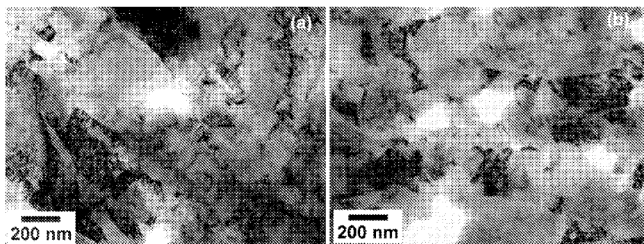
FIG. 36 Bright-field TEM micrographs of microstructure in the 50 mm thick Alloy 8 plate after hot rolling and heat treatment: (a) before and (b) after tensile deformation.
