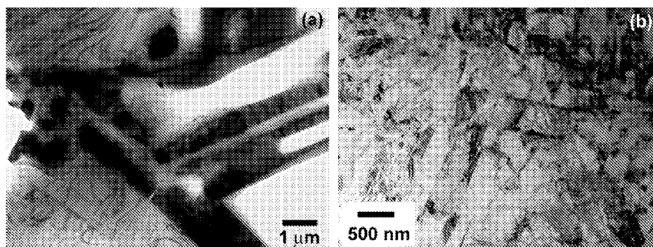
FIG. 42 Bright-field TEM micrographs of microstructure in the 50 mm thick as-cast plate from Alloy 24.
