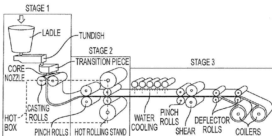
FIG. 2 Thin slab casting process flow diagram showing steel sheet production steps. Note that the process can be broken up into 3 process stages as shown.
