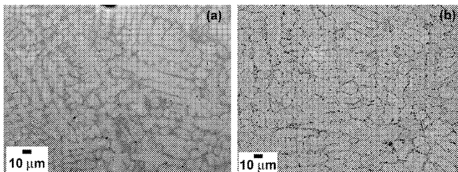
FIG. 16 SEM backscattered electron images of microstructure in the Alloy 59 plate cast at 10 mm thickness (a) as-cast and (b) after HIP.
