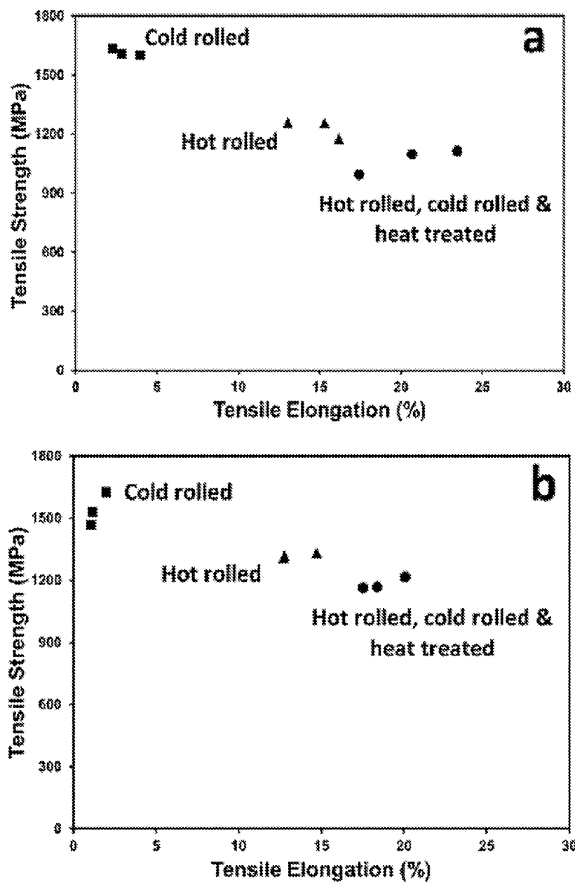
FIG. 27 Tensile properties of (a) Alloy 1 and (b) Alloy 2 after hot rolling, cold rolling, and heat treatment.
