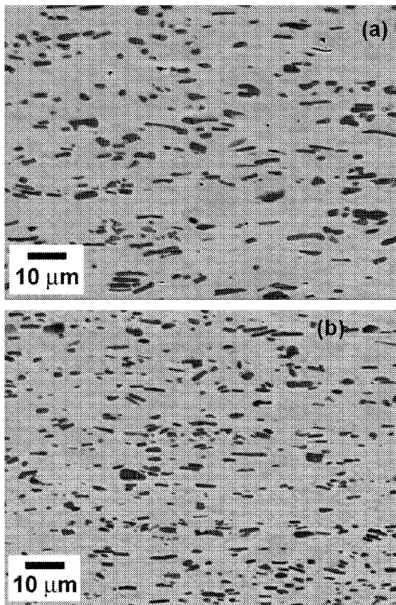
FIG. 22 Backscattered SEM images of microstructure in Alloy 1 plate with as-cast thickness of 10 mm after hot rolling with 88.5% reduction in (a) outer layer region and (b) central layer region.
