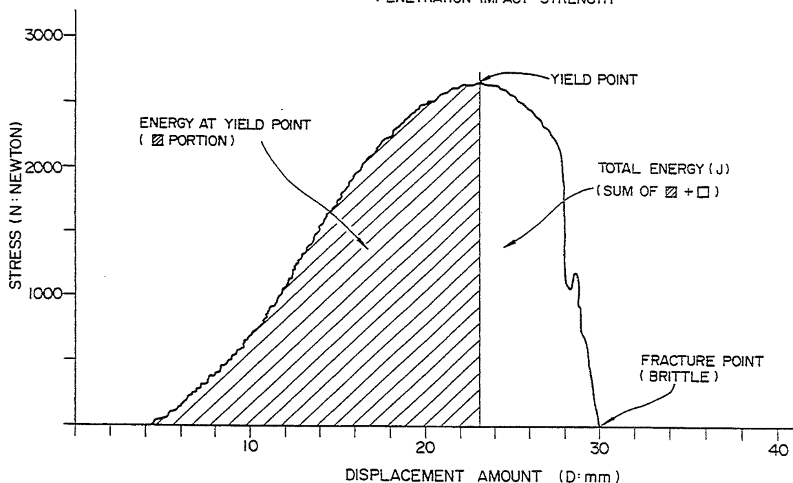
MEASUREMENT OF PENETRATION IMPACT STRENGTH
