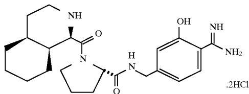
(1R, 4aR, 8aR)-1-Piq-Pro-NHCH 2 C 6 H 3 -3-OH-4-C(NH)NH 2 .2HCl
