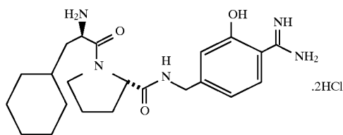
D-Cha-Pro-NHCH 2 C 6 H 3 -3-OH-4-C(NH)NH 2 .2HCl
