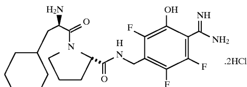
D-Cha-Pro-NHCH 2 C 6 F 3 -3-OH-4-C(NH)NH 2 .2HCl
