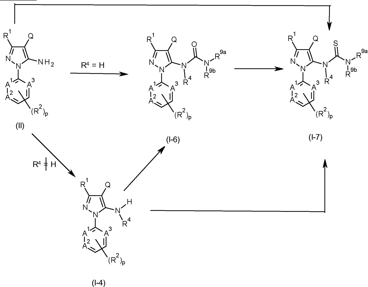
Scheme 4
