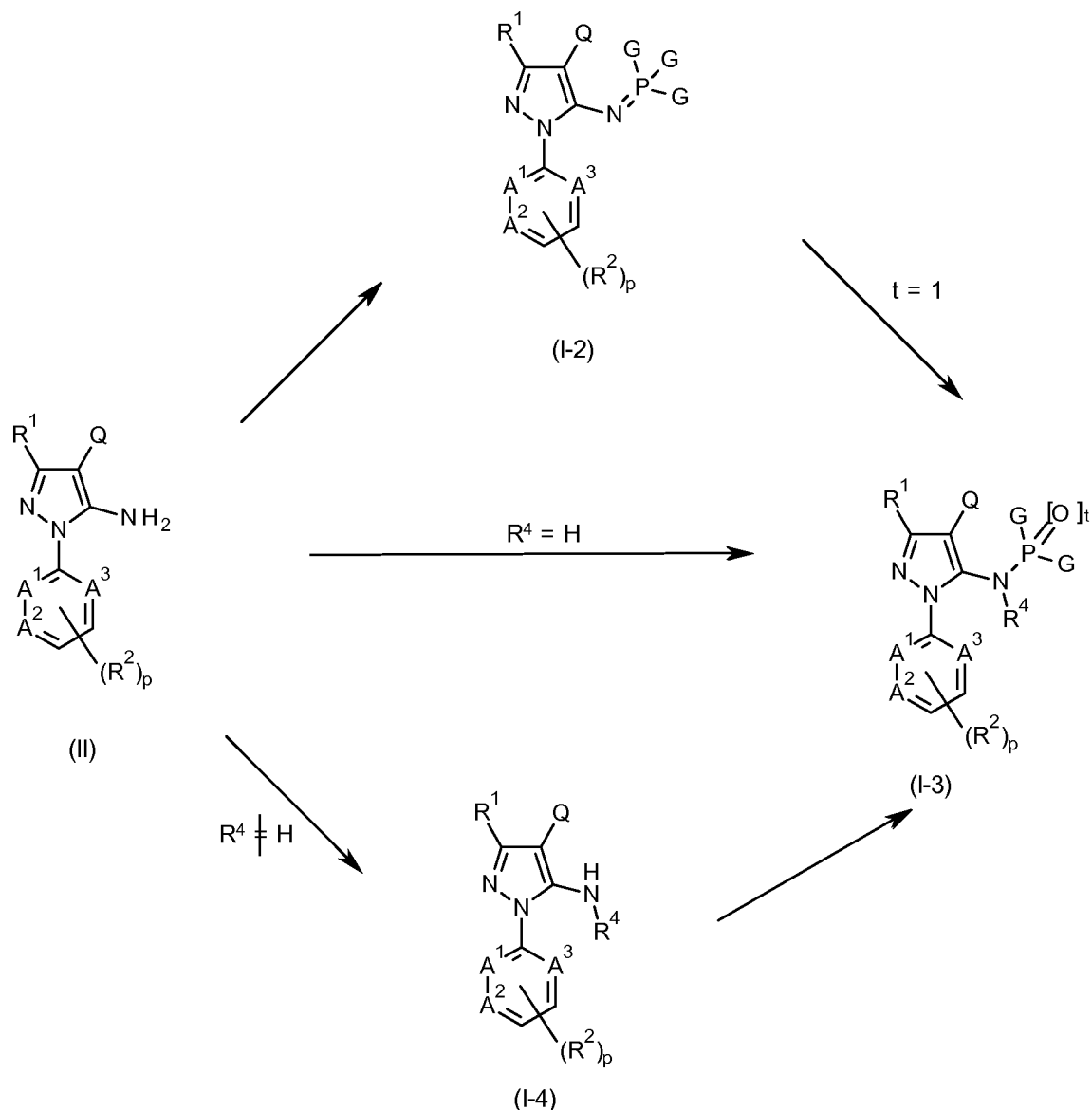
Scheme 2
