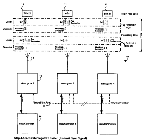
Step-Locked Interrogator Cluster (Internal Sync Signal)
