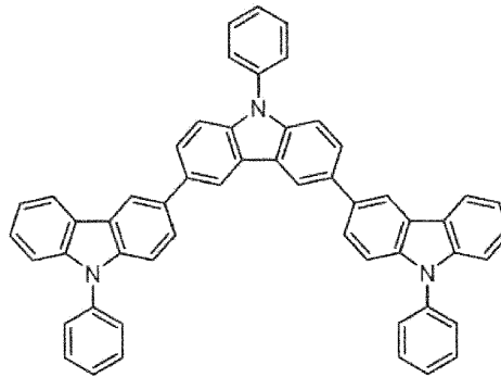
TrisPCz
