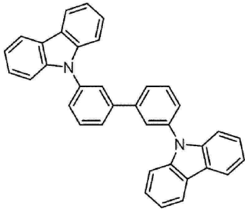
mCBP
