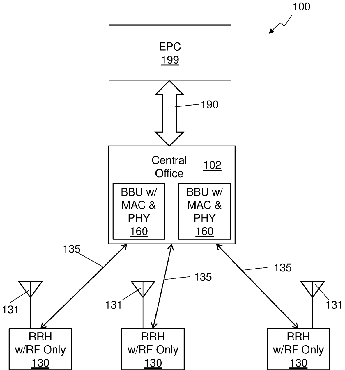
FIG. 1 (PRIOR ART)
