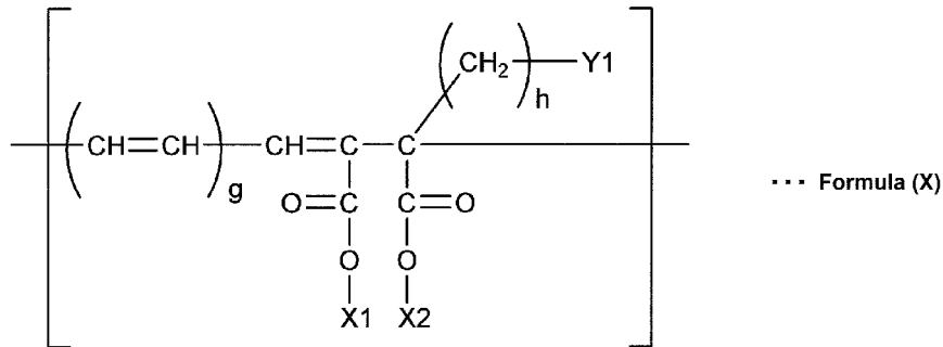
[Chemical 1]
