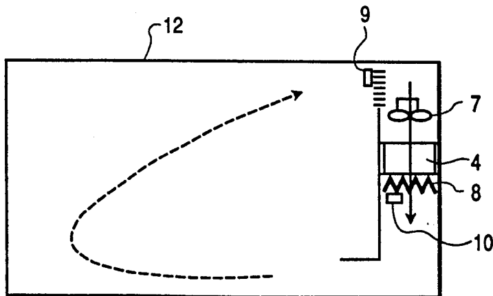
FIG. 4 PRIOR ART
