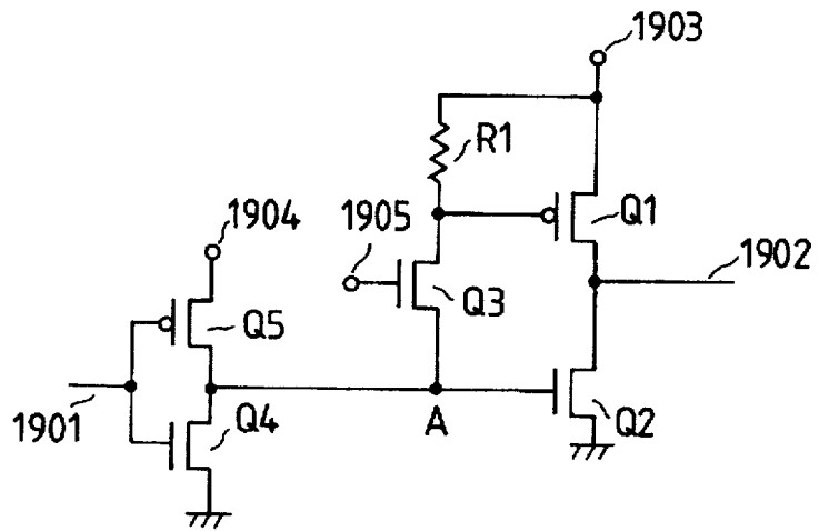
FIG. 19 PRIOR ART
