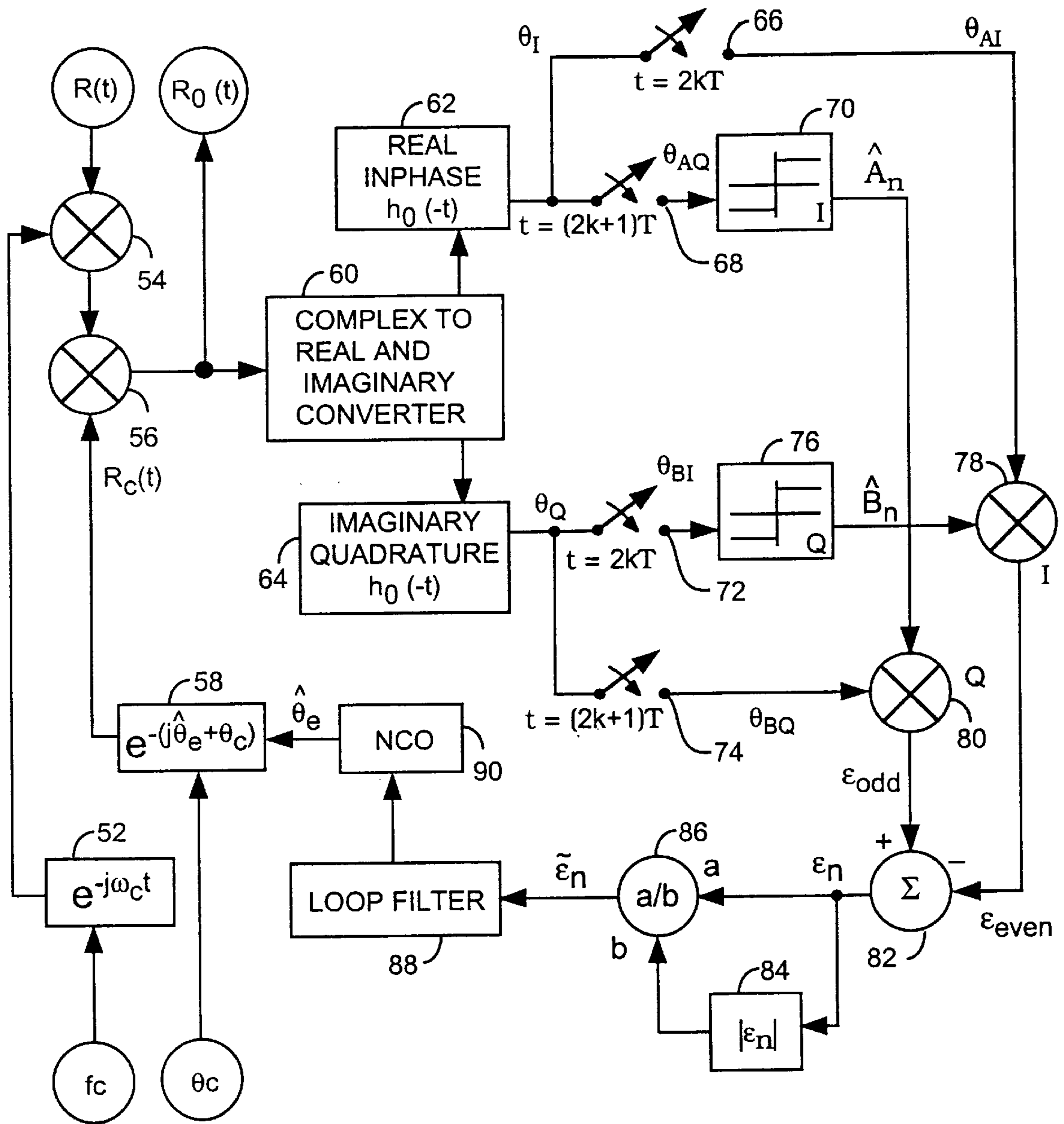
PRECODED GMSK CARRIER TRACKING LOOP
