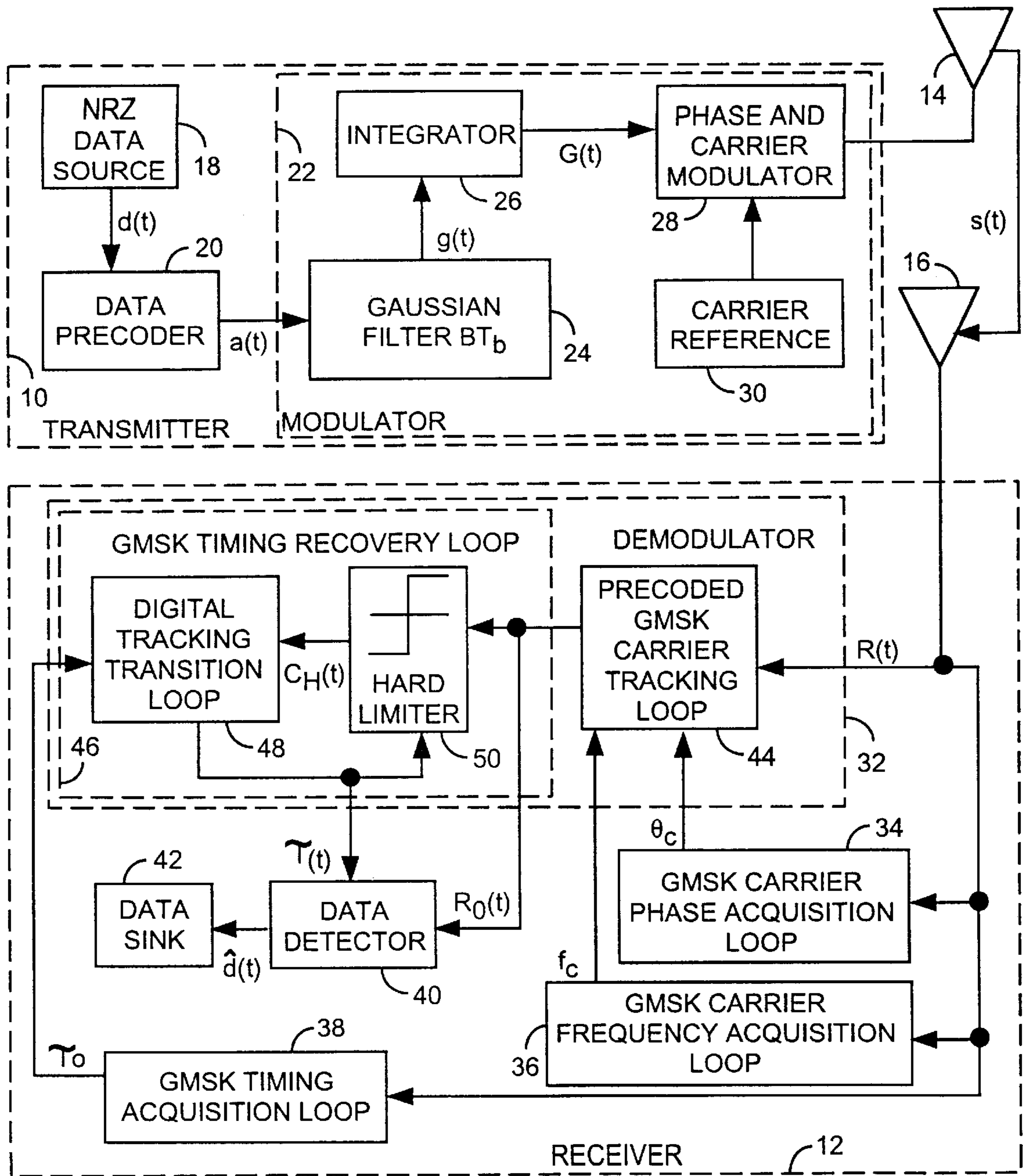
PRECODED GSMK COMMUNICATION SYSTEM
