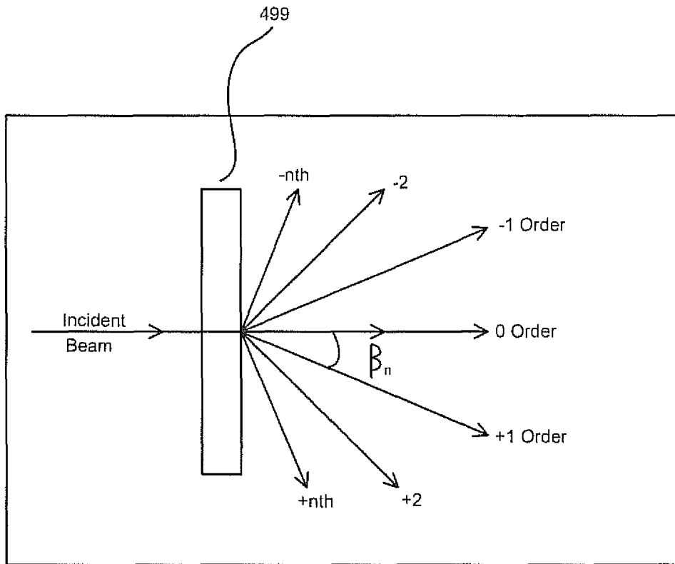
Transmission Grating Diffracted Orders
