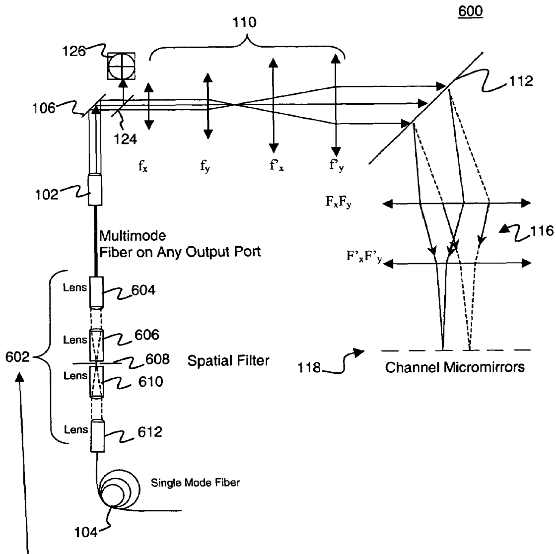
Relay with Spatial Filtering at the Fourier Plane
