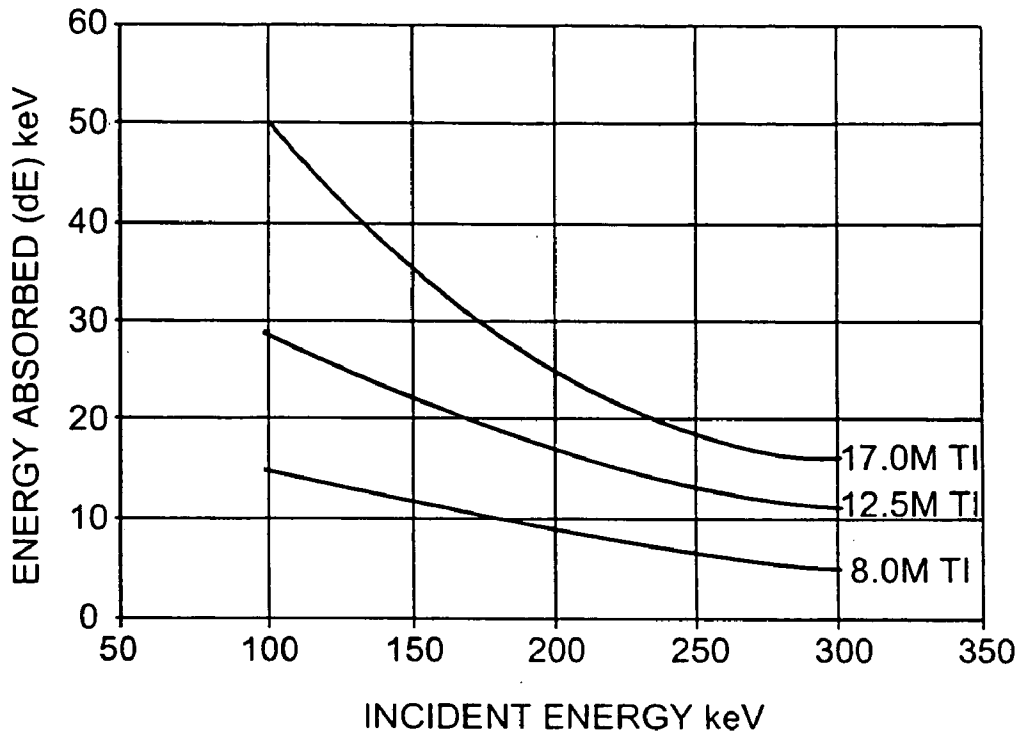
ENERGY ABSORBED FOR VARIOUS THICKNESS TITANIUM FOIL, AS A FUNCTION OF ITS INCIDENT ENERGY (HIGH VOLTAGE)
