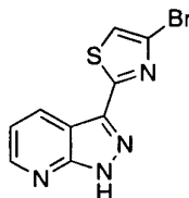
4-Bromo-2-(1H-pyrazolo[3,4b]pyridin-3-yl)thiazole
