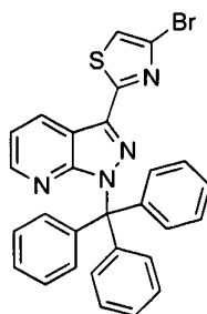
4-Bromo-2-(1-trityl-1H-pyrazolo[3,4-b]pyridin-3-yl)thiazole
