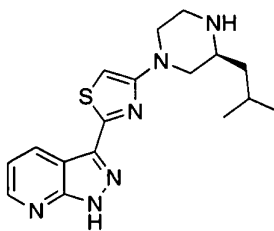
(S)-4-(3-isobutylpiperazin-1-yl)-2-(1H-pyrazolo[3,4-b]pyridin-3-yl)thiazole
