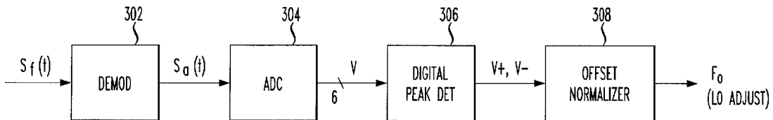
BLOCK DIAGRAM OF NEW AFC BASED ON OFFSET NORMALIZER
