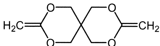
3,9-divinyl-2,4,8,10-tetraoxy-spiro[5.5]undecane
