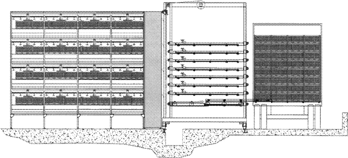
RETRIEVE STACK FROM TRAILER -- HYDRAULIC CYLINDERS PULL STACK INTO RACK ONTO CONVEYOR
