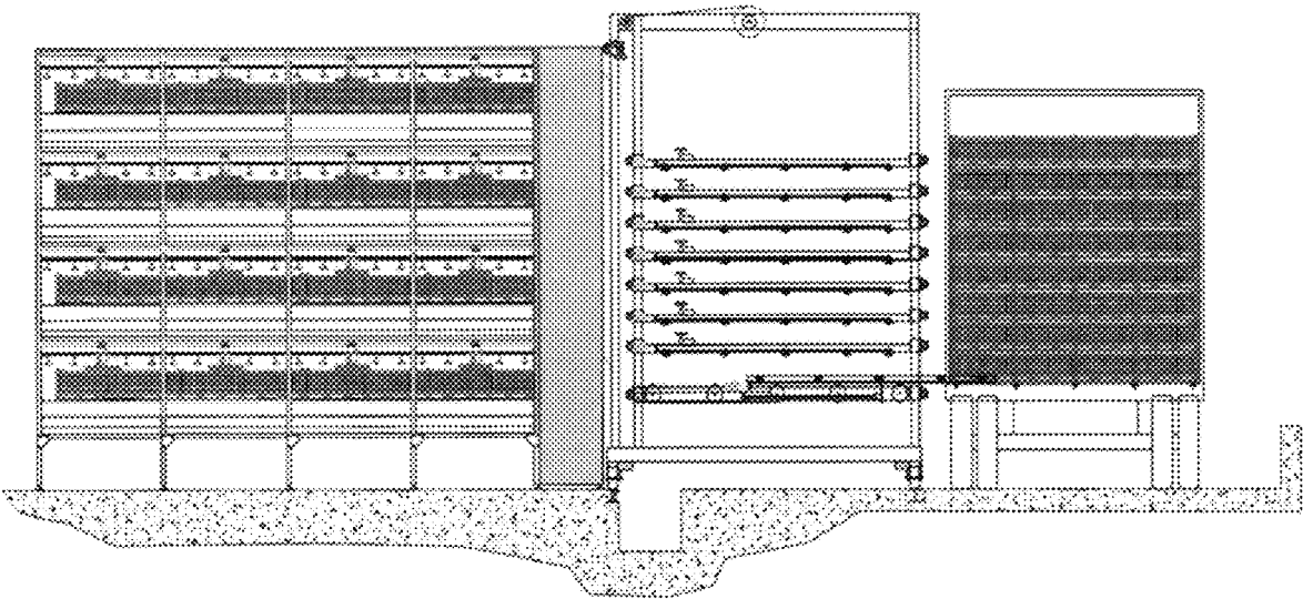
COMPLETE STACK LOADING WITH HYDRAULIC CYLINDERS
