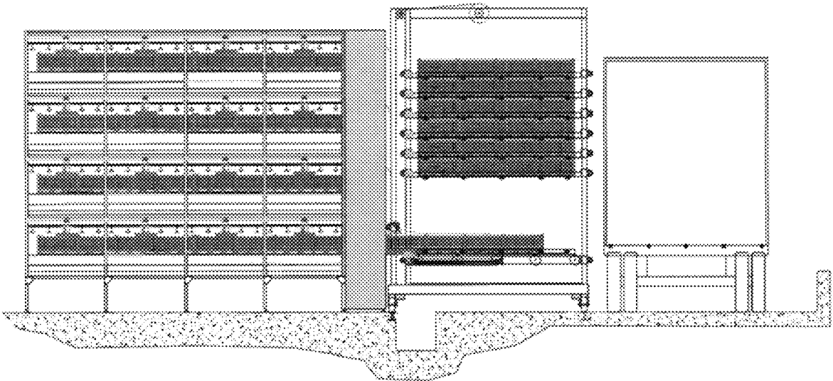
LOAD EIGHTH BASKET FROM LEVEL 1 ON CONVEYOR
