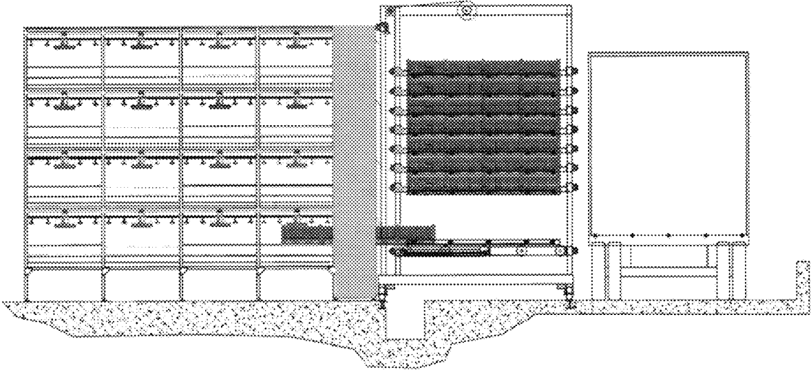
FIG. 22: FILLING RACKS IN ANY ORDER WITH CONVEYOR AND RACK CONVEYANCE.
