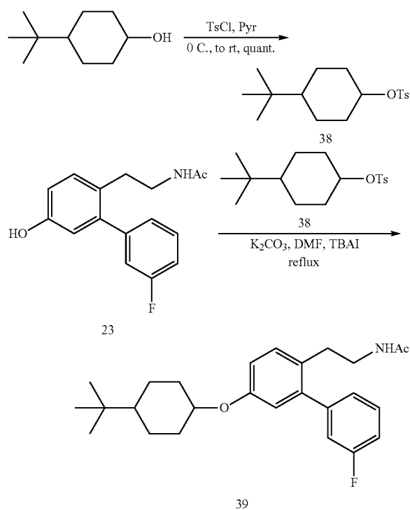
Scheme 8. Synthesis of carbocyclic compound 39.
