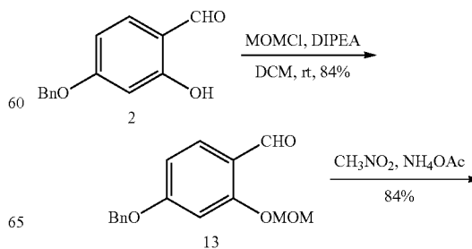
Scheme 4. Synthesis of cyclohexene containing novologues.
