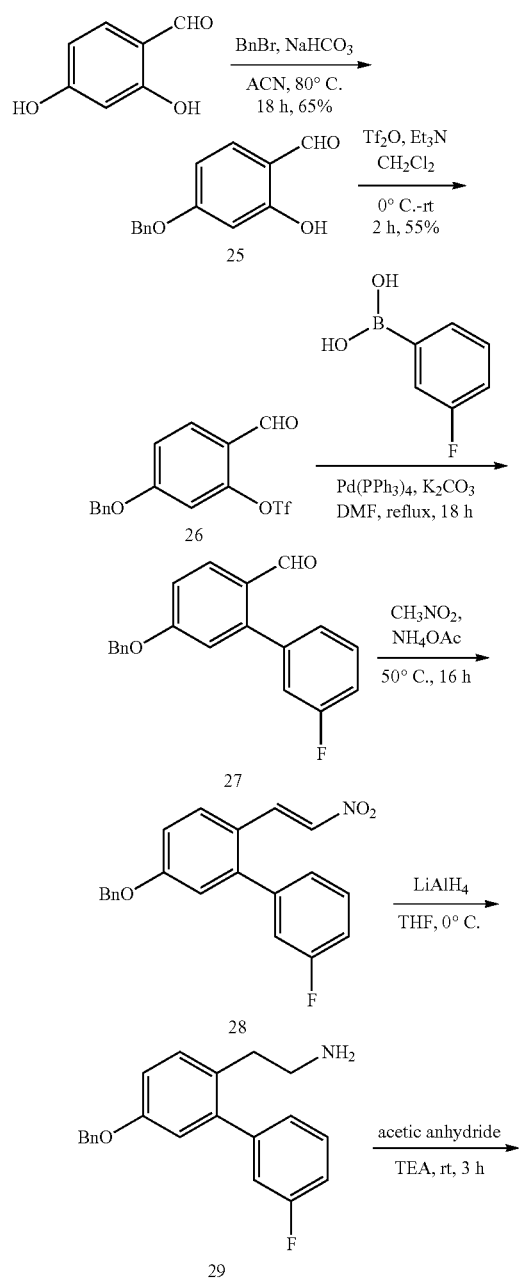
Scheme 6. Synthesis of phenol core intermediate 23.
