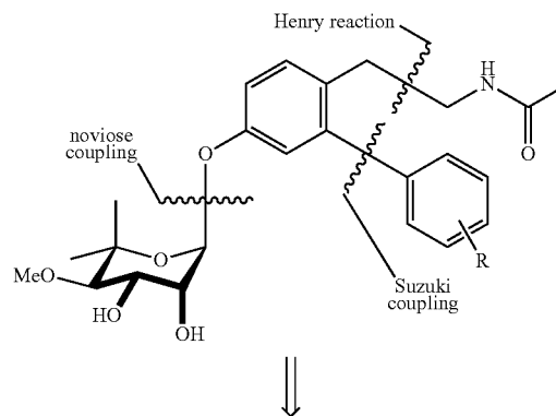
Scheme 1. Retrosynthetic analysis for the construction of novologue.
