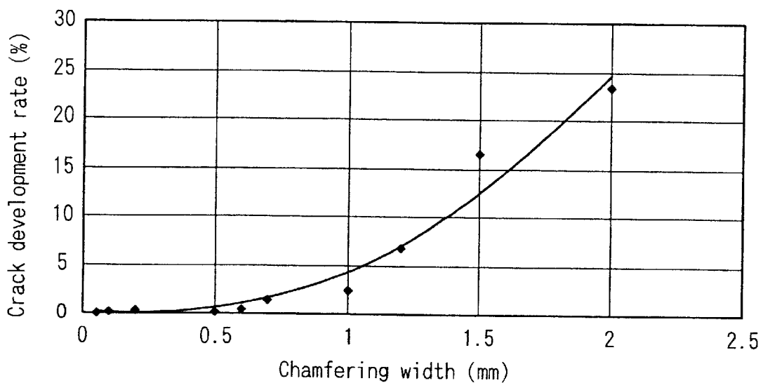
Chamfering width h and Crack development rate
