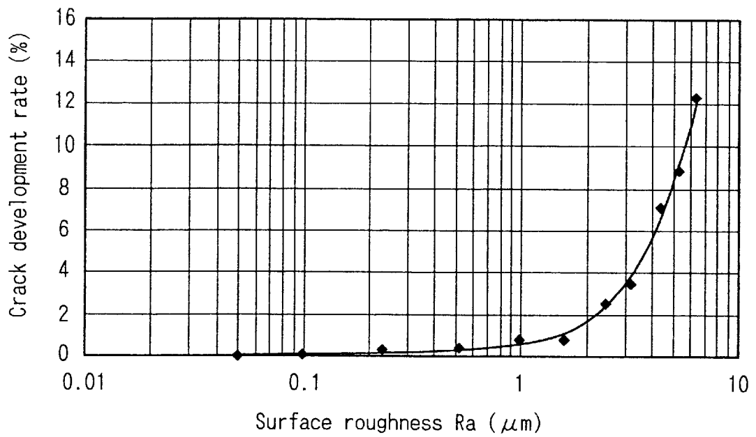
Surface roughness Ra and Crack development rate
