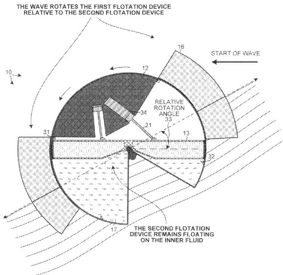
PROPAGATING WAVE ROTATES THE WAVE ENERGY EXTRACTOR COUNTER CLOCKWISE AROUND THE CENTER LOCATION
