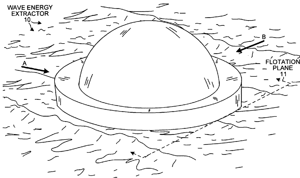
WAVE ENERGY EXTRACTOR IN THE OCEAN FIG. 1
