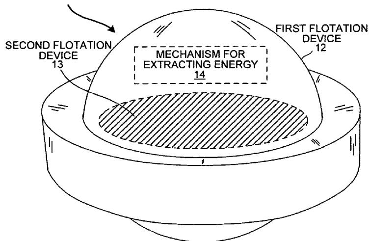
WAVE ENERGY EXTRACTOR FIG. 2
