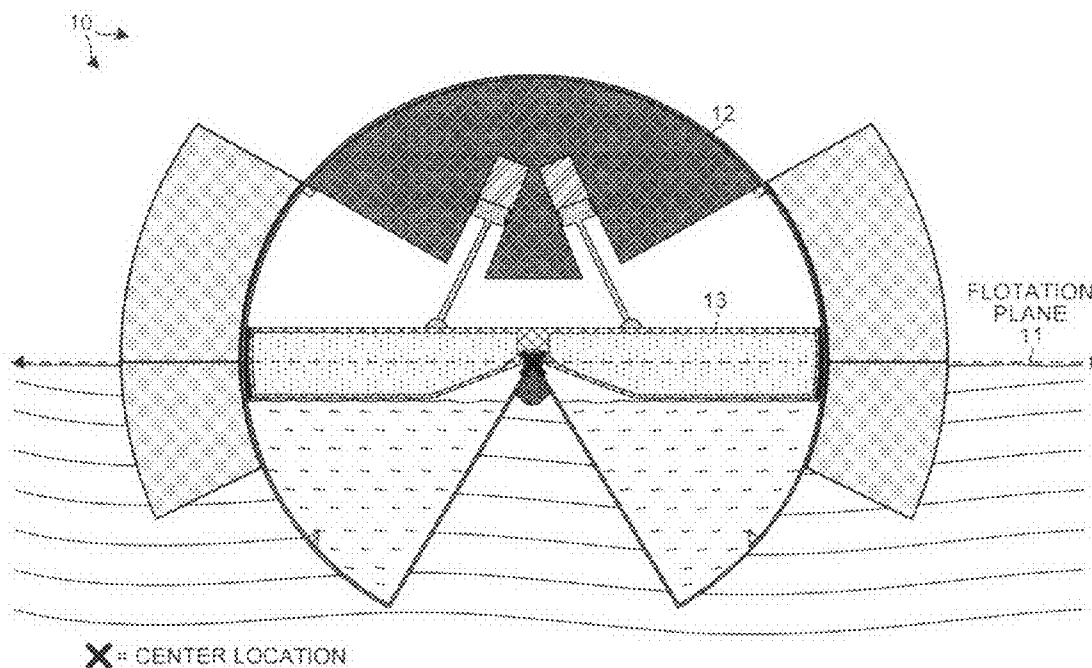
WAVE ENERGY EXTRACTOR IN OCEAN BEFORE ARRIVAL OF AN INCOMING WAVE FIG. 6
