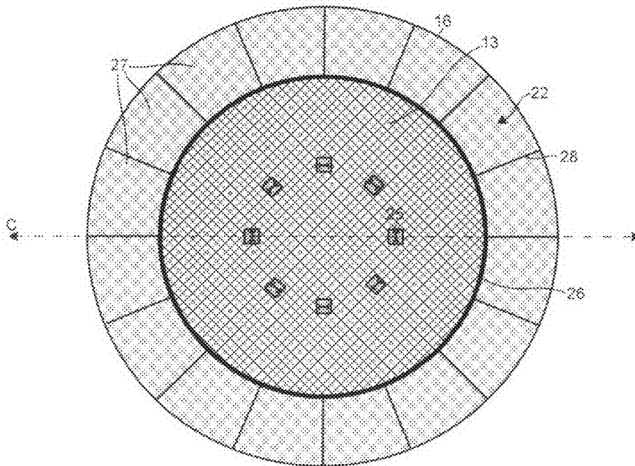
TOP CROSS SECTION OF WAVE ENERGY EXTRACTOR IN THE OCEAN
