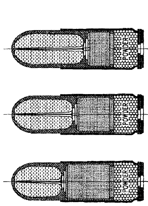
FIG. 1B COLLAPSULE VARIATIONS UTILIZING FREE SPACE
