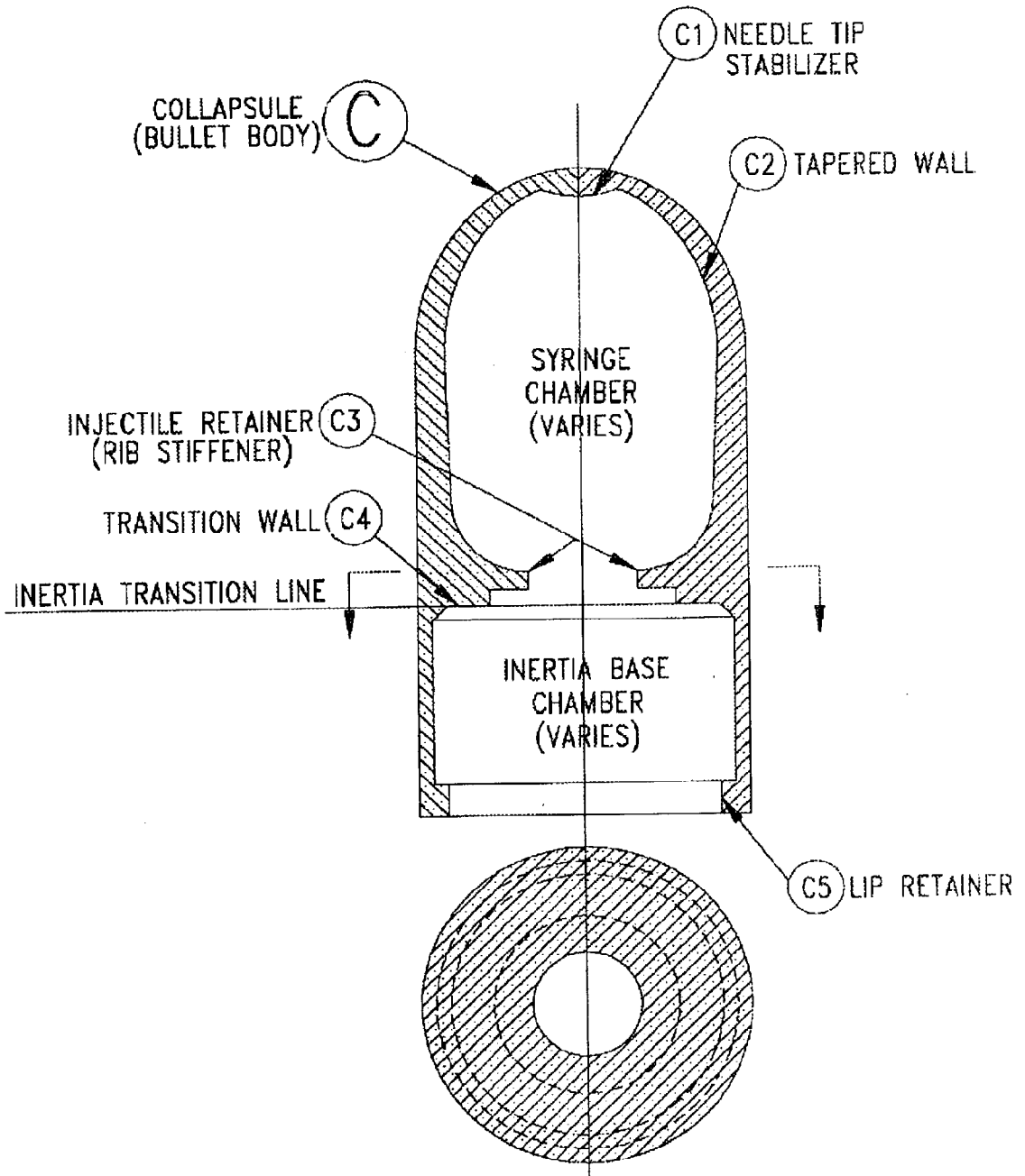
FIG. 4 COLLAPSULE SHELL TAPERED HEAD/TAPERED WALL
