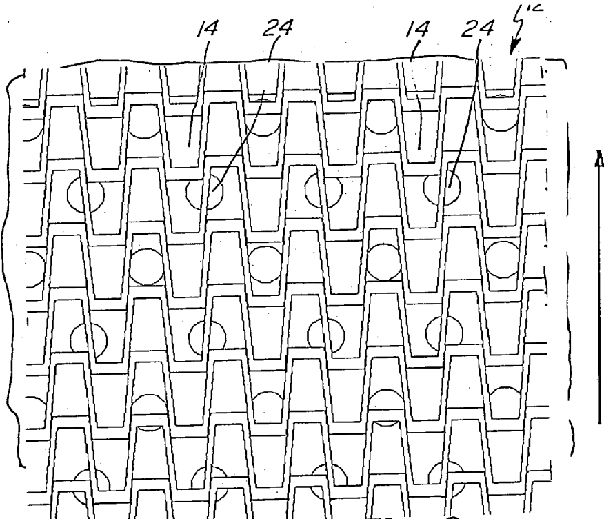
Fig. 9. PRIOR ART
