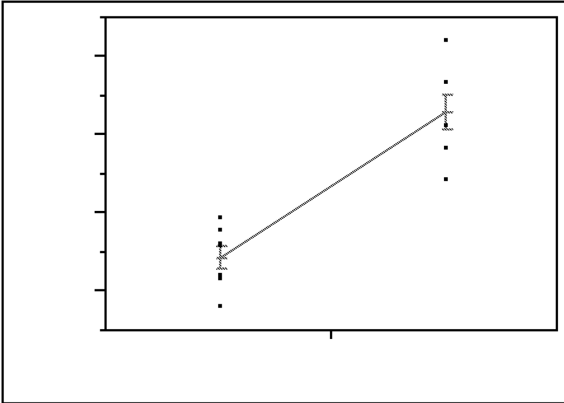
Oneway Analysis of Log2Area By Group ProteinName=SRPG1, PeptideSequence=SGAGTELSVR
