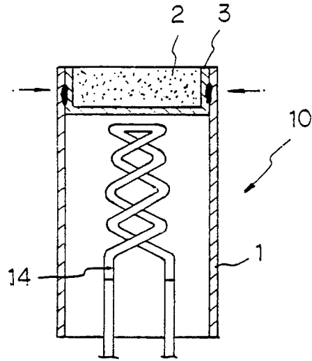
FIG. 2 PRIOR ART
