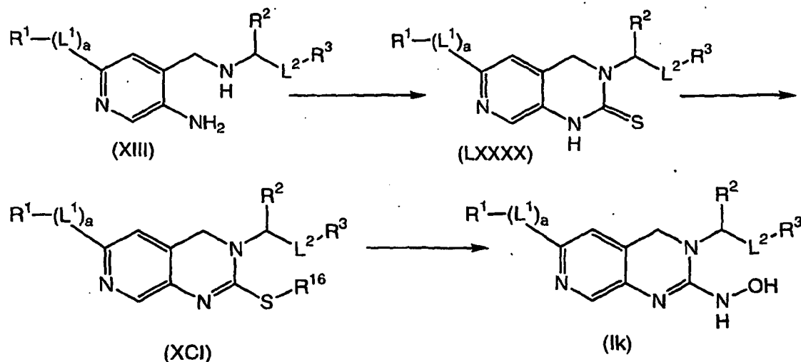
Scheme 14
