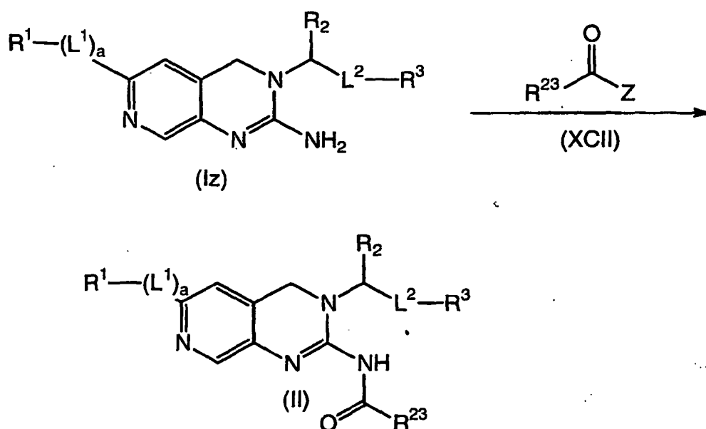
Scheme 16
