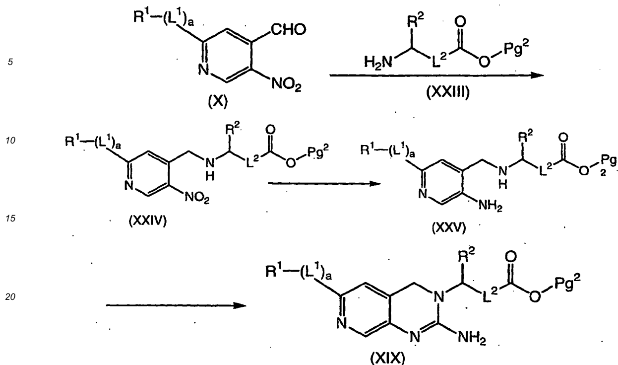
Scheme 4
