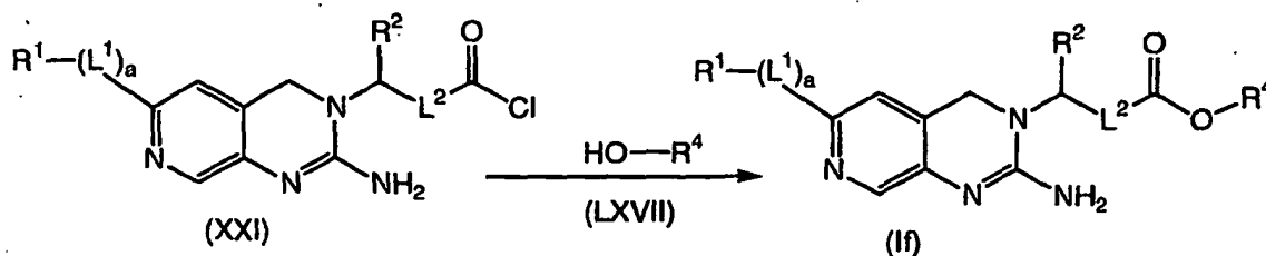
Scheme 9
