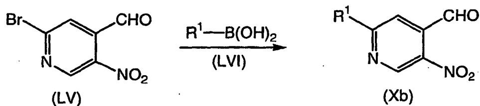
Scheme 6
