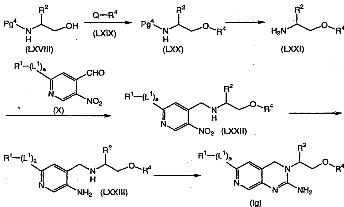
Scheme 10
