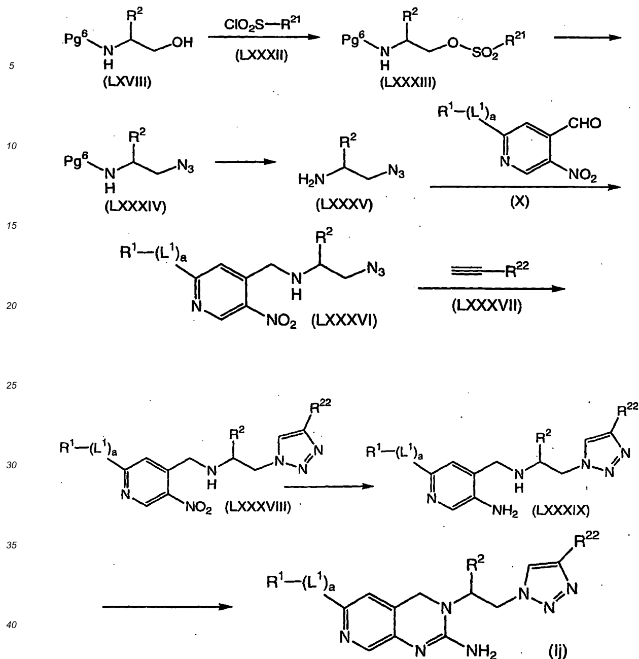
Scheme 13
