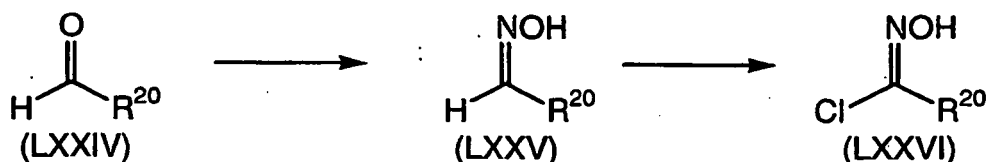
Scheme 12
