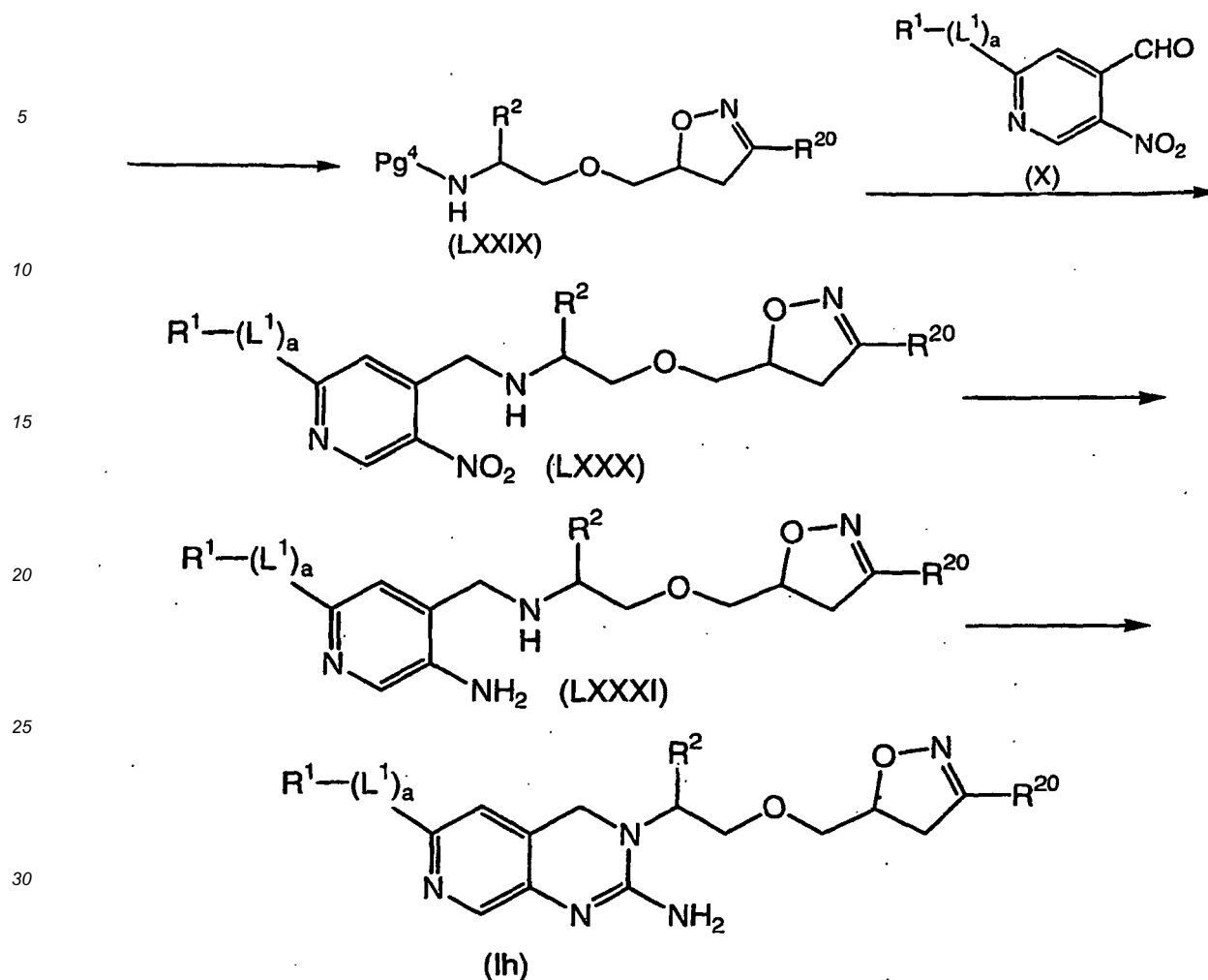
Scheme 11
