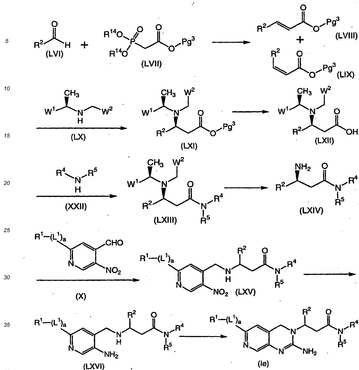
Scheme 8
