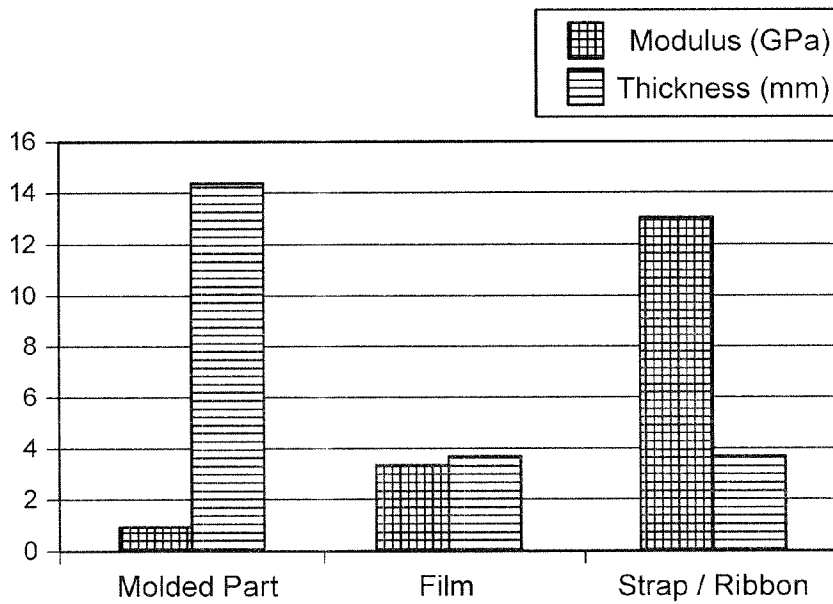
Thickness and Modulus for Equal Load & Width
