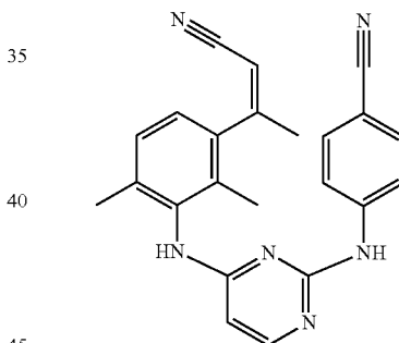
compound 12 = (E) compound 13 = (Z)
