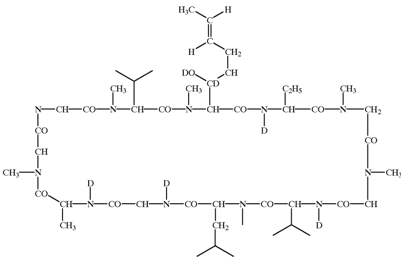
CYCLOSPORIN d-5
