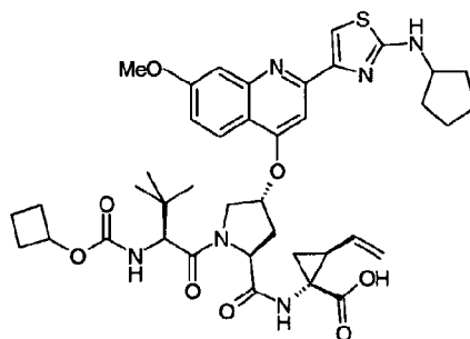
Compound 104
