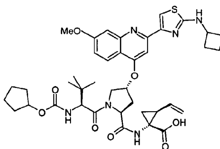
Compound 101
