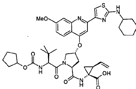
Compound 102
