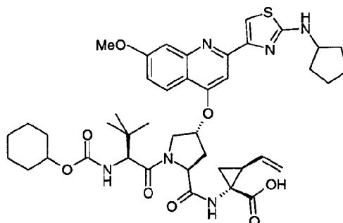
Compound 105
