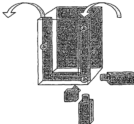
CDD detection system: The 3 CCD detector plates are positioned on orthogonal axis in Cartesian co-ordinate system around the flow cell
