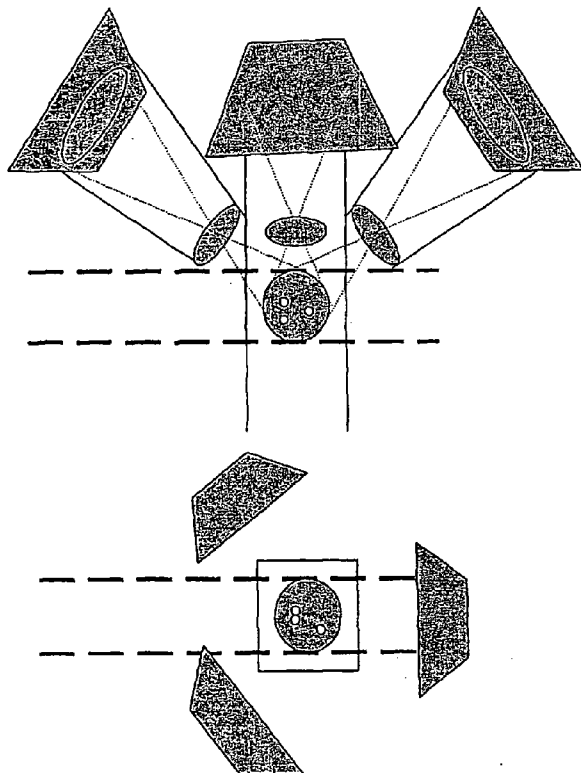
CDD detection system: The 3 CCD detector plates are positioned on orthogonal axis in Cartesian co-ordinate system around the flow cell
