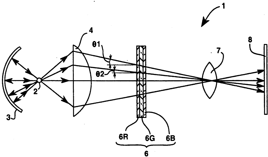
FIG. 6 PRIOR ART
