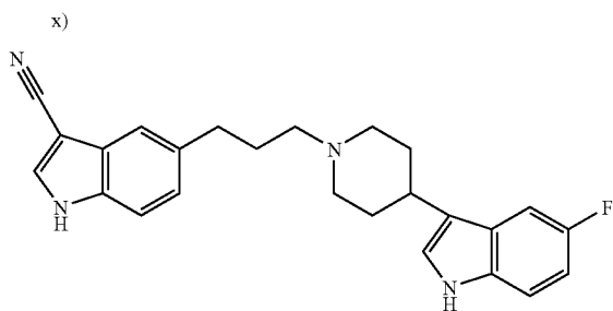
[0251] 5-{3-[4-(5-Fluoro-1H-indol-3-yl)propyl]piperidin-1-yl}propyl-1H-indole-3-carbonitrile
