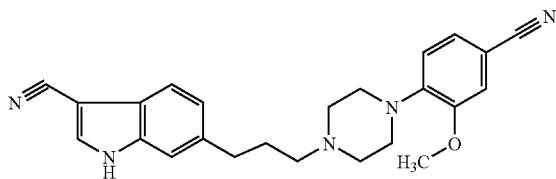
[0259] 6-{3-[4-(4-Cyano-2-methoxyphenyl)piperazin-1-yl]propyl}-1H-indole-3-carbonitrile
