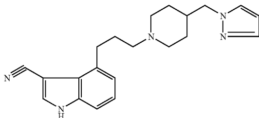
[0260] 4-[3-(4-Pyrazol-1-ylmethyl-1-piperidyl)propyl]-1H-indole-3-carbonitrile
