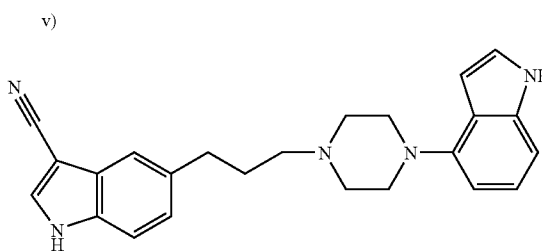
[0249] 5-[3-[4-(1H-Indol-4-yl)piperazin-1-yl]propyl]-1H-indole-3-carbonitrile
