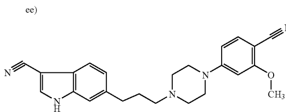
[0258] 6-{3-[4-(4-Cyano-3-methoxyphenyl)piperazin-1-yl]propyl}-1H-indole-3-carbonitrile
