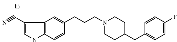
[0235] 5-{3-[4-(4-Fluorobenzyl)-1-piperidyl]propyl}-1H-indole-3-carbonitrile;
