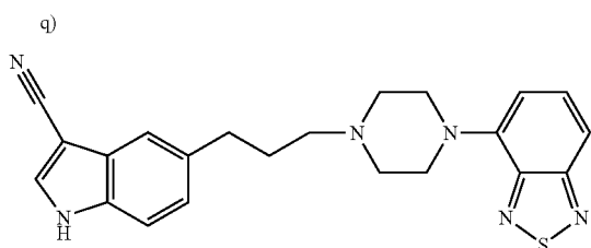
[0244] 5-[3-(4-Benzo[1,2,5]thiadiazol-4-yl)piperazin-1-yl]propyl]-1H-indole-3-carbonitrile
