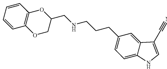
[0265] 5-{3-[(2,3-Dihydrobenzo[1,4]dioxin-2-ylmethyl)amino]propyl}-1H-indole-3-carbonitrile
