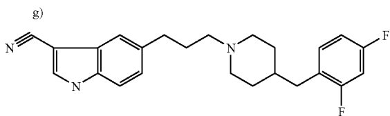
[0234] 5-{3-[4-(2,4-Difluorobenzyl)-1-piperidyl]propyl}-1H-indole-3-carbonitrile;
