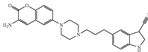
[0273] 5-{3-[4-(3-Amino-2-oxo-2H-chromen-6-yl)piperazin-1-yl]propyl}-1H-indole-3-carbonitrile
