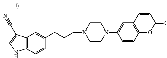
[0239] 5-{3-[4-(2-Oxo-2H-chromen-6-yl)piperazin-1-yl]propyl}-1H-indole-3-carbonitrile
