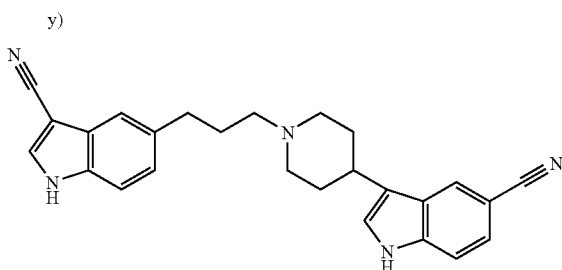
[0252] 3-{1-[3-(3-Cyano-1H-indol-5-yl)propyl]piperidin-4-yl}-1H-indole-5-carbonitrile
