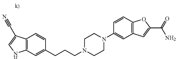
[0238] 5-{4-[3-(3-Cyano-1H-indol-6-yl)propyl]piperazin-1-yl}benzofuran-2-carboxamide
