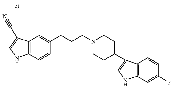
[0253] 5-{3-[4-(6-Fluoro-1H-indol-3-yl)propyl]piperidin-1-yl}propyl-1H-indole-3-carbonitrile
