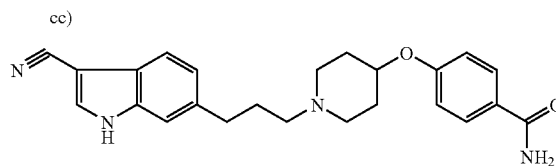
[0256] 4-{1-[3-(3-Cyano-1H-indol-6-yl)propyl]piperidin-4-yloxy}benzamide
