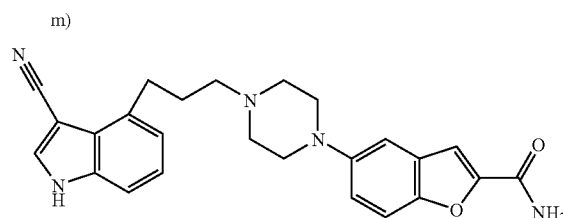
[0240] 5-{4-[3-(3-Cyano-1H-indol-4-yl)propyl]piperazin-1-yl}benzofuran-2-carboxamide
