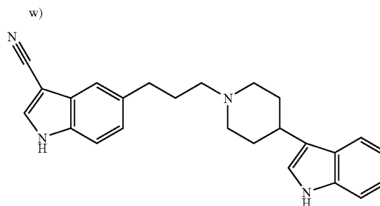
[0250] 5-[3-[4-(1H-Indol-3-yl)piperidin-1-yl]propyl]-1H-indole-3-carbonitrile
