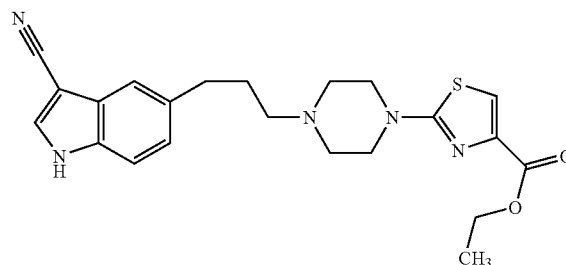
[0270] Ethyl 2-[4-[3-(3-cyano-1H-indol-5-yl)propyl]piperazin-1-yl]-thiazole-4-carboxylate
