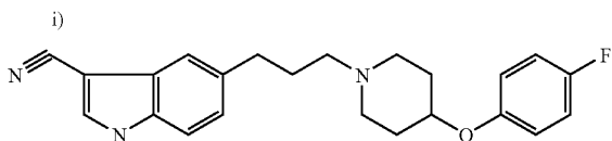
[0236] 5-{3-[4-(4-Fluorophenoxy)-1-piperidyl]propyl}-1H-indole-3-carbonitrile;
