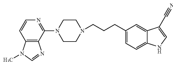
[0267] 5-{3-[4-(1-Methyl-1H-imidazo[4,5-c]pyridin-4-yl)piperazin-1-yl]propyl}-1H-indole-3-carbonitrile
