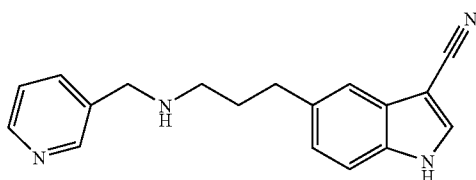
[0262] 5-{3-[(Pyridin-3-ylmethyl)amino]propyl}-1H-indole-3-carbonitrile
