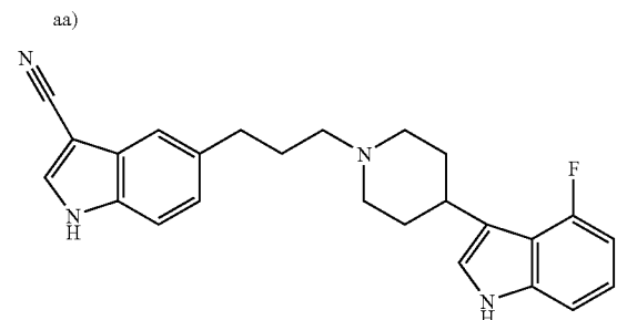
[0254] 5-{3-[4-(4-Fluoro-1H-indol-3-yl)propyl]piperidin-1-yl}propyl-1H-indole-3-carbonitrile
