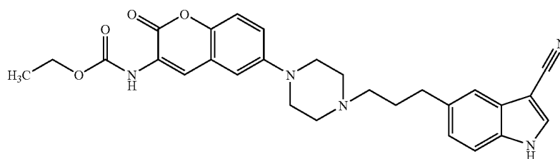
[0272] Ethyl (6-{4-[3-(3-Cyano-1H-indol-5-yl)propyl]piperazin-1-yl}-2-oxo-2H-chromen-3-yl)carbamate
