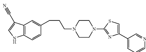
[0269] 5-{3-[4-(4-Pyridin-3-ylthiazol-2-yl)piperazin-1-yl]propyl}-1H-indole-3-carbonitrile
