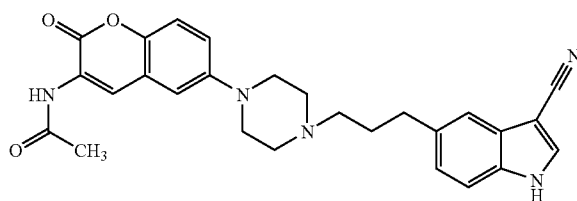
[0261] N-(6-{4-[3-(3-Cyano-1H-indol-5-yl)propyl]piperazin-1-yl}-2-oxo-2H-chromen-3-yl)acetamide
