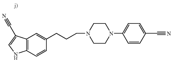
[0237] 5-{3-[4-(4-Cyanophenyl)piperazin-1-yl]propyl}-1H-indole-3-carbonitrile
