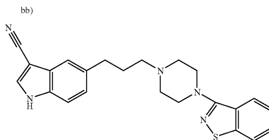
[0255] 5-[3-(4-Benzo[d]isothiazol-3-yl)piperazin-1-yl]propyl-1H-indole-3-carbonitrile
