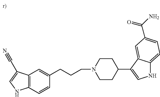
[0245] 3-{1-[3-(3-Cyano-1H-indol-5-yl)propyl]piperidin-4-yl}-1H-indole-5-carboxamide
