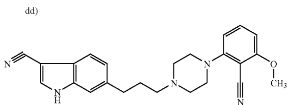
[0257] 6-{3-[4-(2-Cyano-3-methoxyphenyl)piperazin-1-yl]propyl}-1H-indole-3-carbonitrile
