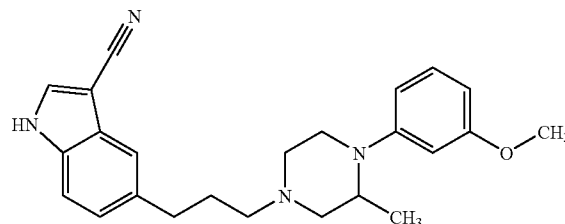
[0266] 5-{3-[4-(3-Methoxyphenyl)-3-methylpiperazin-1-yl]propyl}-1H-indole-3-carbonitrile
