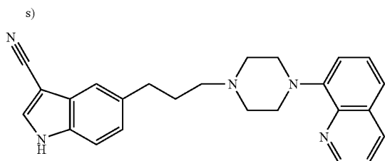
[0246] 5-[3-(4-Quinolin-8-yl)piperazin-1-yl]propyl]-1H-indole-3-carbonitrile
