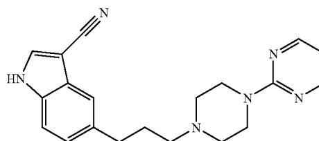
[0264] 5-[3-(4-Pyrimidin-2-ylpiperazin-1-yl)propyl]-1H-indole-3-carbonitrile
