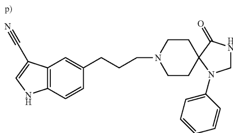
[0243] 5-[3-(4-Oxo-1-phenyl-1,3,8-triazaspiro[4.5]dec-8-yl)propyl]-1H-indole-3-carbonitrile
