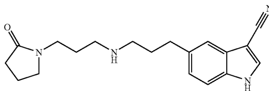
[0271] 5-{3-[3-(2-Oxopyrrolidin-1-yl)propylamino]propyl}-1H-indole-3-carbonitrile
