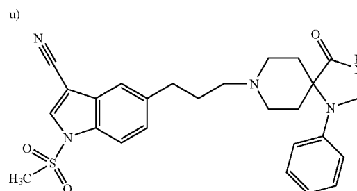
[0248] 1-Methanesulfonyl-5-[3-(4-oxo-1-phenyl-1,3,8-triazaspiro[4.5]dec-8-yl)propyl]-1H-indole-3-carbonitrile
