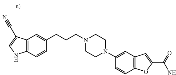
[0241] 5-{4-[3-(3-Cyano-1H-indol-5-yl)propyl]piperazin-1-yl}benzofuran-2-carboxamide
