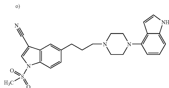
[0242] 5-{3-[4-(1H-Indol-4-yl)piperazin-1-yl]propyl}-1-methanesulfonyl-1H-indole-3-carbonitrile
