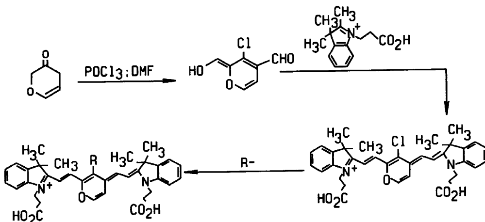
Synthesis of "tunable" cyanine dyes
