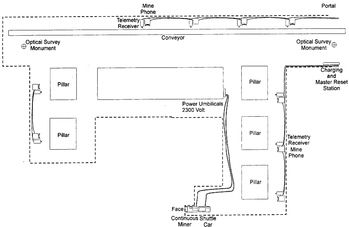
Note: Drawing is not to scale.
