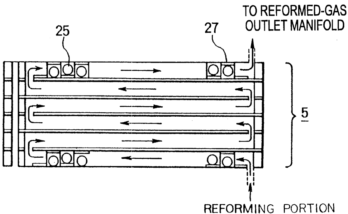
5: MULTILAYER CO OXIDATION PORTION
