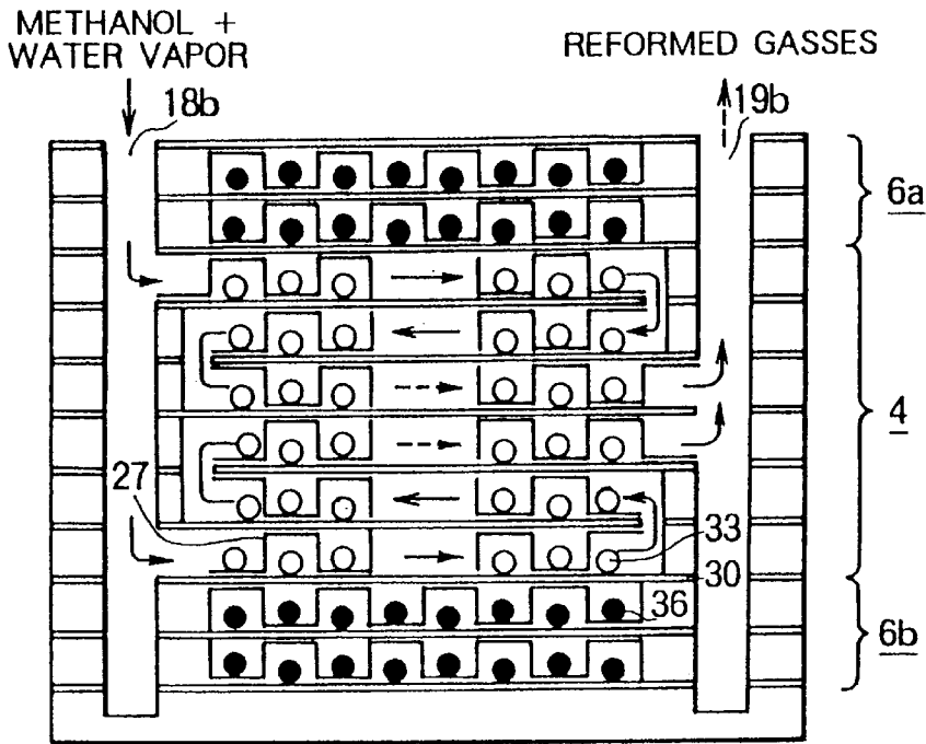
4: MULTILAYER REFORMING PORTION 6a,6b: CATALYTIC COMBUSTION PORTIONS
