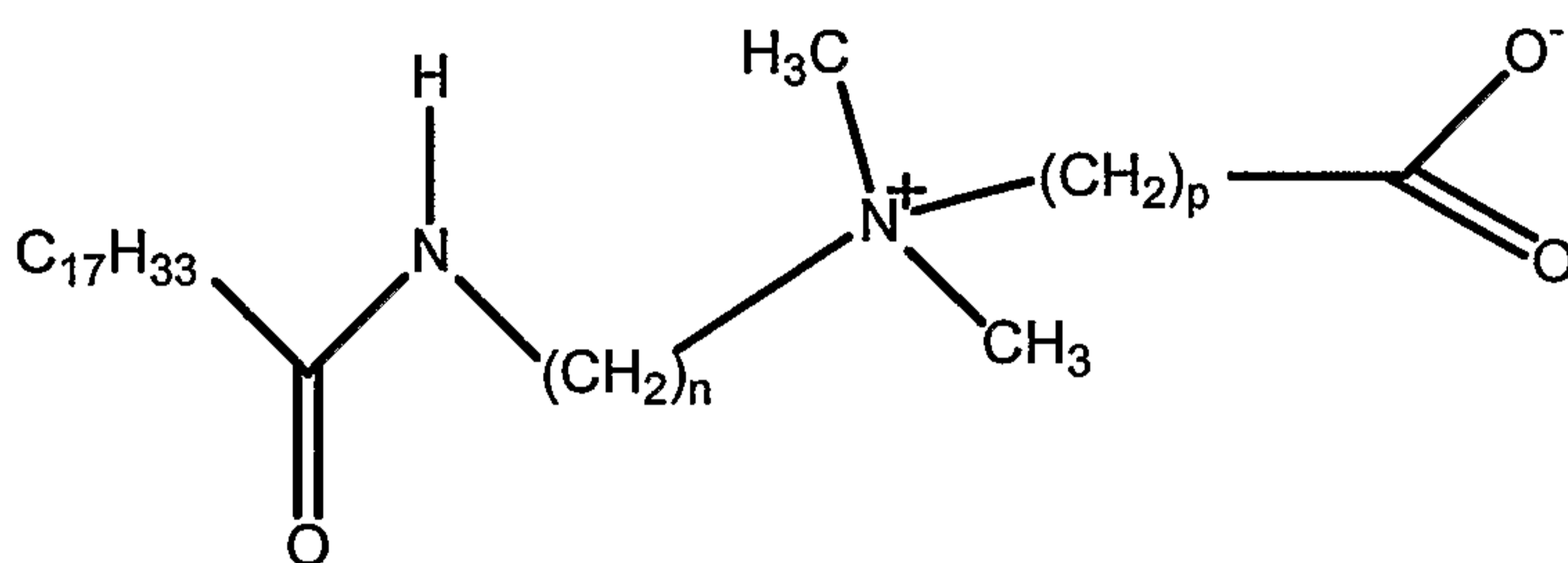
Surfactant in BET-O-30 (when n = 3 and p = 1 )
