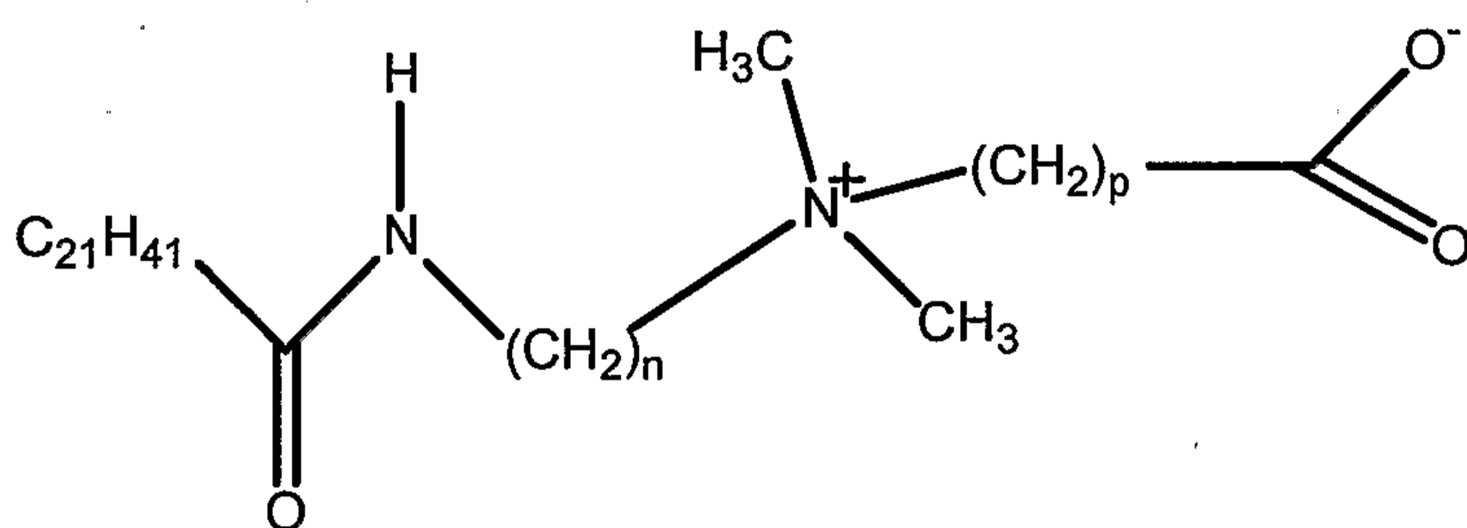
Surfactant in BET-E-40 (when n = 3 and p = 1 )
