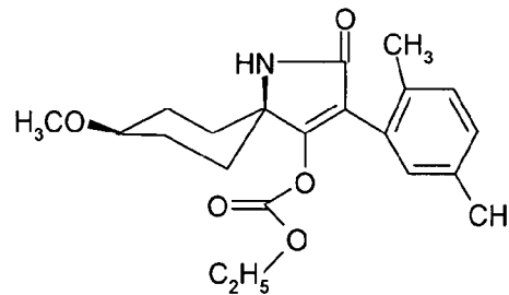
(I-4) Spirotetramat
