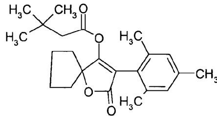
(I-2) Spiromesifen
