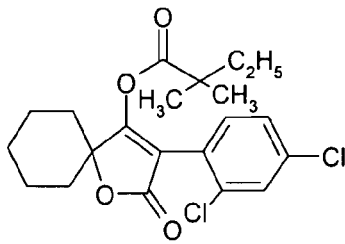
(I-1) Spirodiclofen
