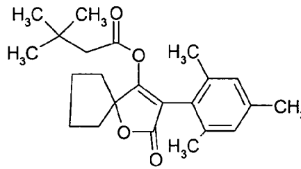
(I-2) Spiromesifen
