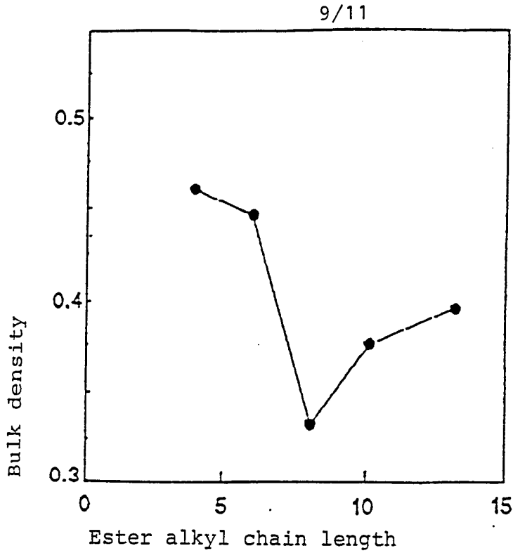
Fig. 18. Bulk density of the polymers as a function of the alkyl group chain length in the donor
