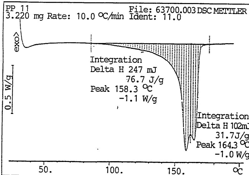
Fig. 21. DSC curve of the polymer PP-C-13
