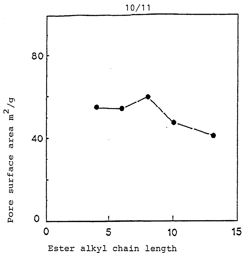
Fig. 23. Pore surface area ( m^2/g ) in the polymers as a function of the alkyl group chain length in the donor
