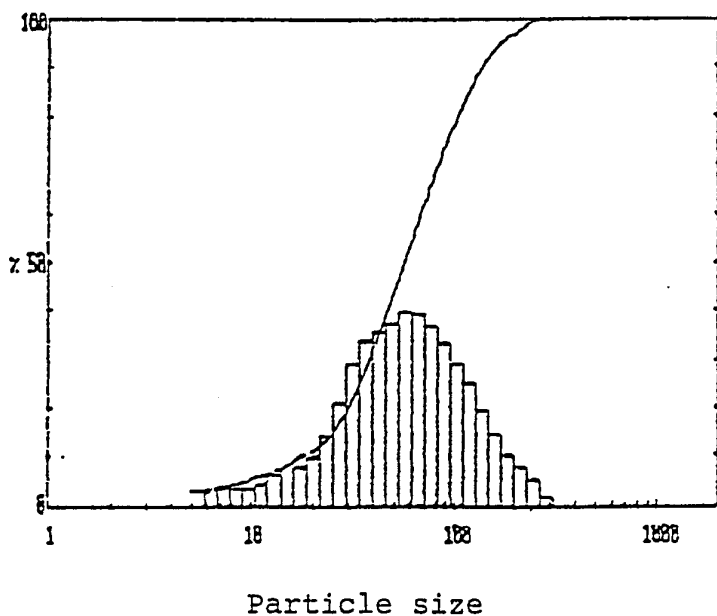
Fig. 6. Catalyst particle size distribution when decyl phthalate (C = 10) was used as an internal donor
