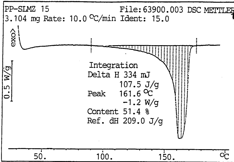
Fig. 19. DSC (differential scanning calorimeter) curve of the polymer PP-C-4
