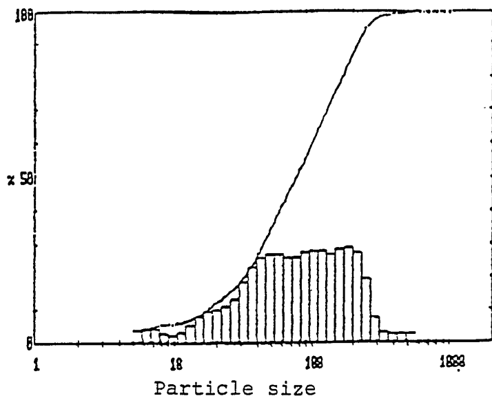
Fig. 5. Catalyst particle size distribution when octyl phthalate (C = 8) was used as an internal donor
