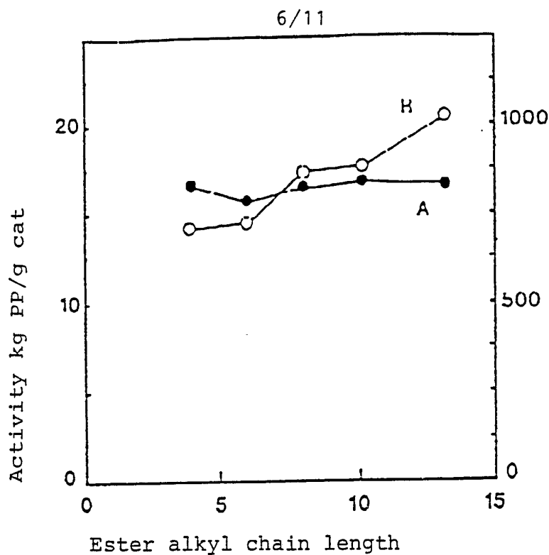
Fig. 13. Catalyst activity as a function of the alkyl group chain length in the donor. Curve (A) refers to the unit kg PP/g cat. and curve (B) to the unit kg PP/g Ti
