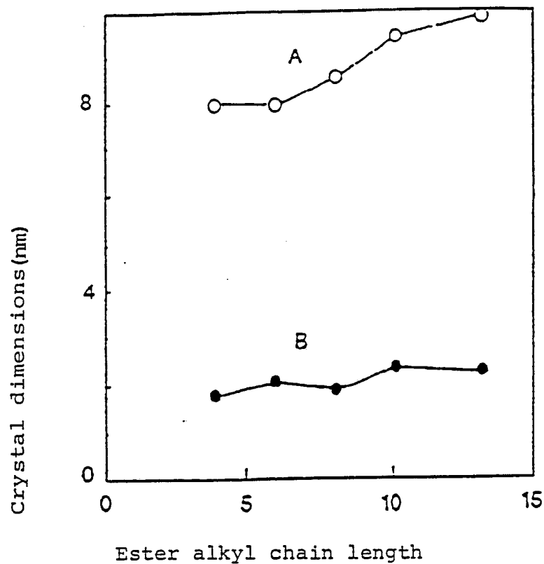
Fig. 11. Width (A) and height (B) of the MgCl_2 crystal as a function of the alkyl group chain length in the donor
