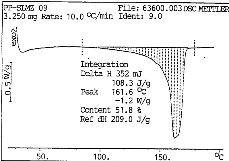
Fig. 20. DSC curve of the polymer PP-C-8
