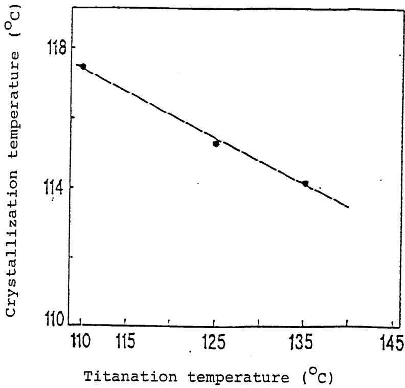
Fig. 22. Crystallization temperature of polypropylene as a function of the titanation ( \text{TiCl}_4 treatment) temperature used in the catalyst synthesis
