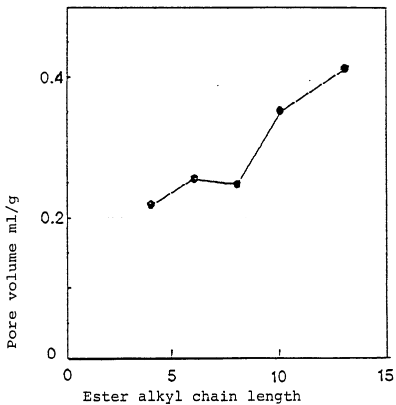
Fig. 24. Pore volume (ml/g) in the polymers as a function of the chain length of the alkyl group in the donor
