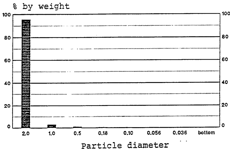
Fig. 15. Particle size distribution of the polymer PP-C-8 (C = 8)
