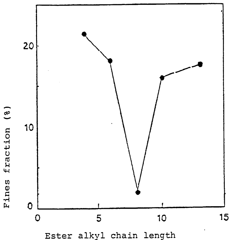
Fig. 17. Total amount of fines fraction ( d < 1\text{mm} ) as a function of the alkyl group chain length in the donor
