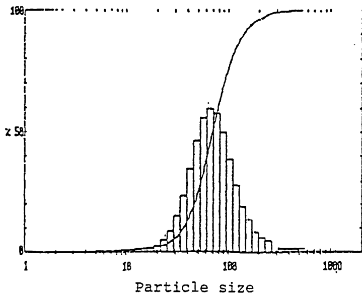
Fig. 7. Catalyst particle size distribution when tri-decyl phthalate (C = 13) was used as an internal donor
