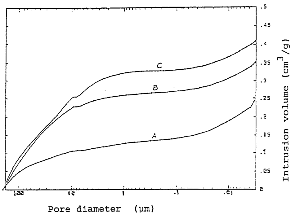
Fig. 25. Pore volume distributions of polymers PP-C-8 (A), PP-C-10 (B) and PP-C-13 (C)
