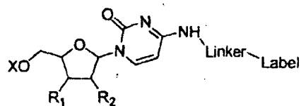
Cytidine N4-linker
