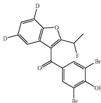
2,6-dibromo-4-[2-(1-fluoroethyl)(5,7- 2 H 2 )-1-benzofuran-3-carbonyl]phenol
