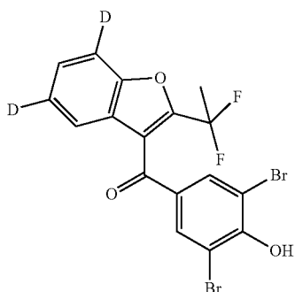
2,6-dibromo-4-[2-(1,1-difluoroethyl)(5,7- 2 H 2 )-1-benzofuran-3-carbonyl]phenol
