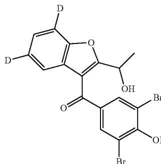
2,6-dibromo-4-[2-(1-hydroxyethyl)(5,6- 2 H 2 )-1-benzofuran-3-carbonyl]phenol
