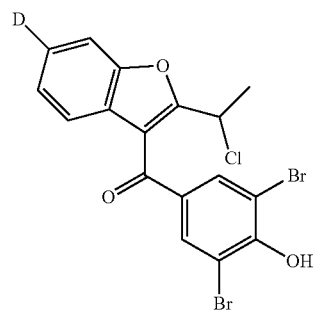
2,6-dibromo-4-[2-(1-chloroethyl)(6- 2 H)-1-benzofuran-3-carbonyl]phenol
