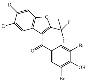
2,6-dibromo-4-[2-(1,1-difluoroethyl)(5,6- 2 H 2 )-1-benzofuran-3-carbonyl]phenol
