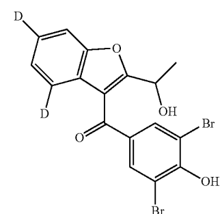
2,6-dibromo-4-[2-(1-hydroxyethyl)(4,6- 2 H 2 )-1-benzofuran-3-carbonyl]phenol
