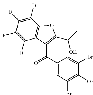
2,6-dibromo-4-[5-fluoro-2-(1-hydroxyethyl)(4,6,7- ^2H_3 )-1-benzofuran-3-carbonyl]phenol
