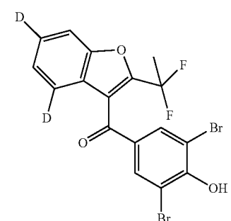
2,6-dibromo-4-[2-(1,1-difluoroethyl)(4,6- 2 H 2 )-1-benzofuran-3-carbonyl]phenol
