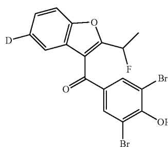
2,6-dibromo-4-[2-(1-fluoroethyl)(5- 2 H)-1-benzofuran-3-carbonyl]phenol
