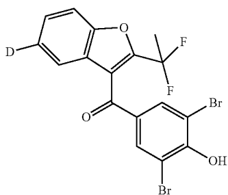
2,6-dibromo-4-[2-(1,1-difluoroethyl)(5- 2 H)-1-benzofuran-3-carbonyl]phenol
