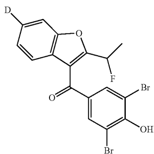
2,6-dibromo-4-[2-(1-fluoroethyl)(6- 2 H)-1-benzofuran-3-carbonyl]phenol
