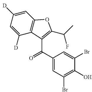
2,6-dibromo-4-[2-(1-fluoroethyl)(4,6- 2 H 2 )-1-benzofuran-3-carbonyl]phenol
