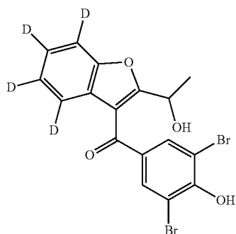
2,6-dibromo-4-[2-(1-hydroxyethyl)(4,5,6,7- ^2H_4 )-1-benzofuran-3-carbonyl]phenol
