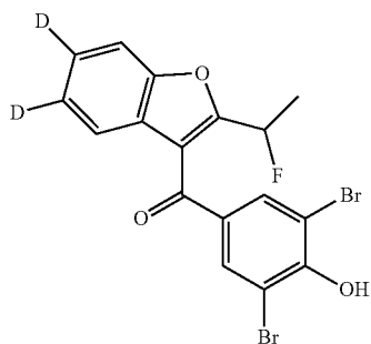
2,6-dibromo-4-[2-(1-fluoroethyl)(5,6- 2 H 2 )-1-benzofuran-3-carbonyl]phenol
