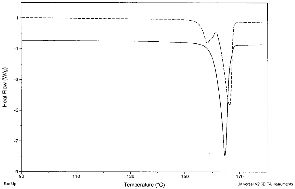
Figure 16: Effect of seeding during precipitation. Dashed line = unseeded sample, solid line = sample seeded with raw material itraconazole. The unseeded trace (dashed line) has been shifted upward by 1.5 W/g for clarity. (Example 17)
