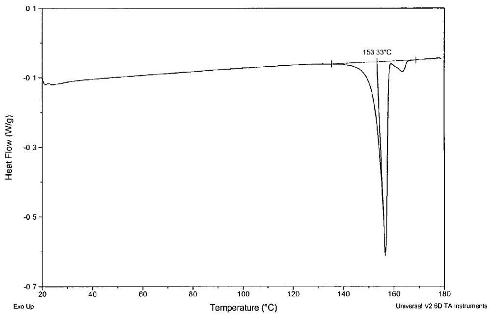
Figure 13b: DSC trace for SMP-2-PRE. (Example 16)
