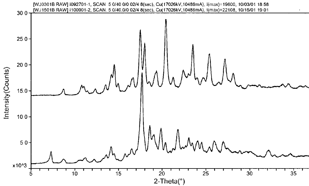
Figure 17: Effect of seeding the drug concentrate through aging. Top x-ray diffraction pattern is for crystals prepared from fresh drug concentrate, and is consistent with the stable polymorph (see Figure 12, top). Bottom pattern is for crystals prepared from aged (seeded) drug concentrate, and is consistent with the metastable polymorph (see Figure 12, bottom). The top pattern has been shifted upward for clarity. (Example 18)
