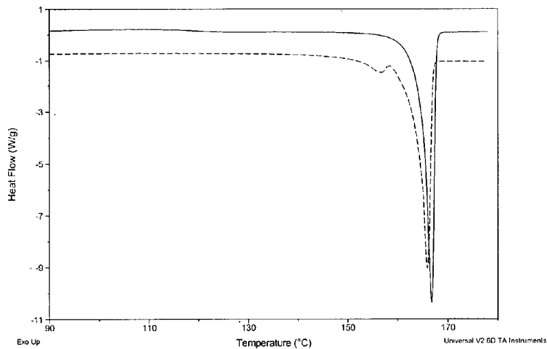
Figure 15: Comparison of SMP-2-PRE samples after homogenization. Solid line = sample seeded with raw material itraconazole. Dashed line = unseeded sample. The solid line has been shifted by 1 W/g for clarity (Example 16)
