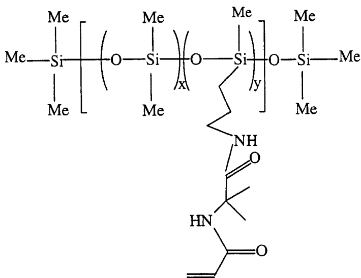
acrylamide-functionalised polydimethyl-aminopropylsiloxane copolymer
